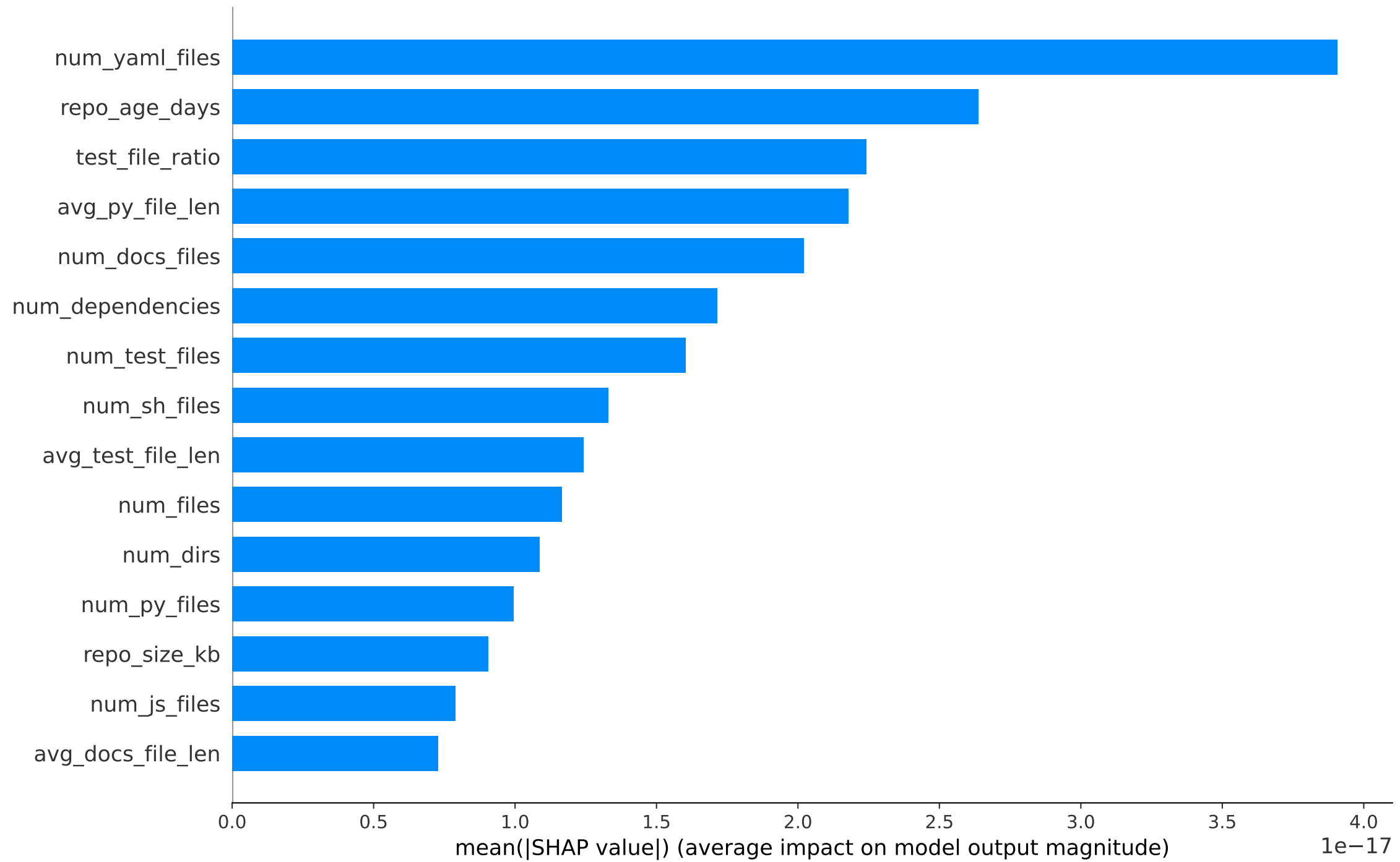
SHAP Mean Absolute Impact (random_forest)
