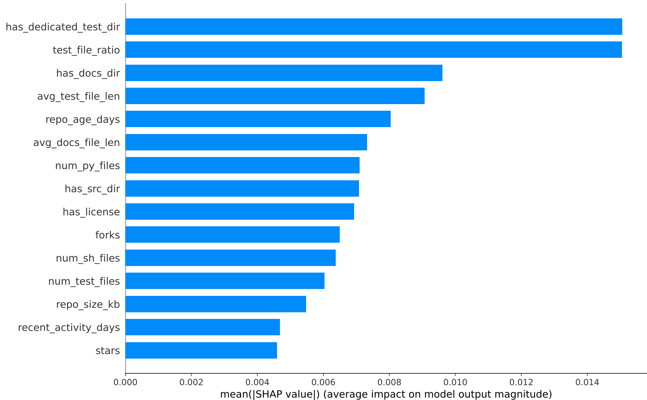
SHAP Mean Absolute Impact (svm)
