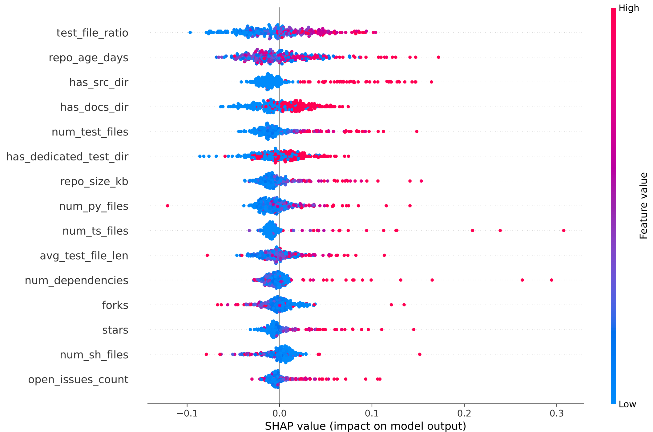
SHAP Feature Importance (neural_network)
