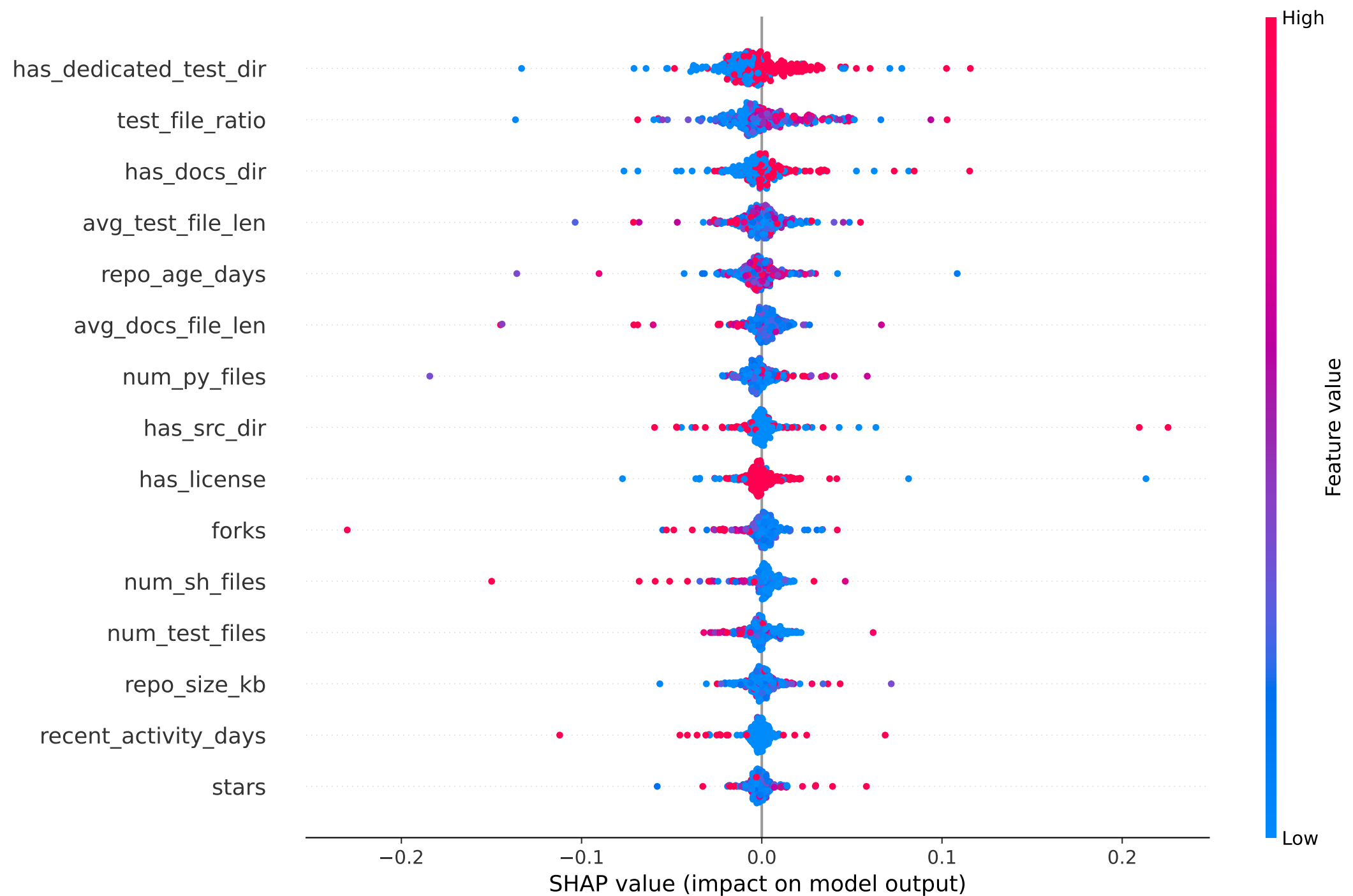
SHAP Feature Importance (svm)
