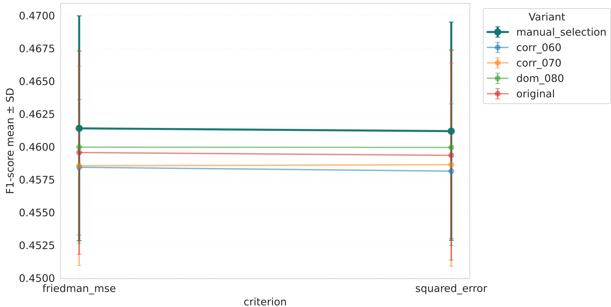
Gradient Boosting by criterion
