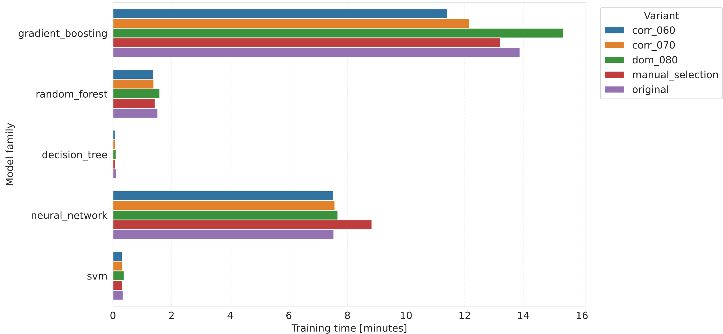
Training-time comparison by variant and model family
