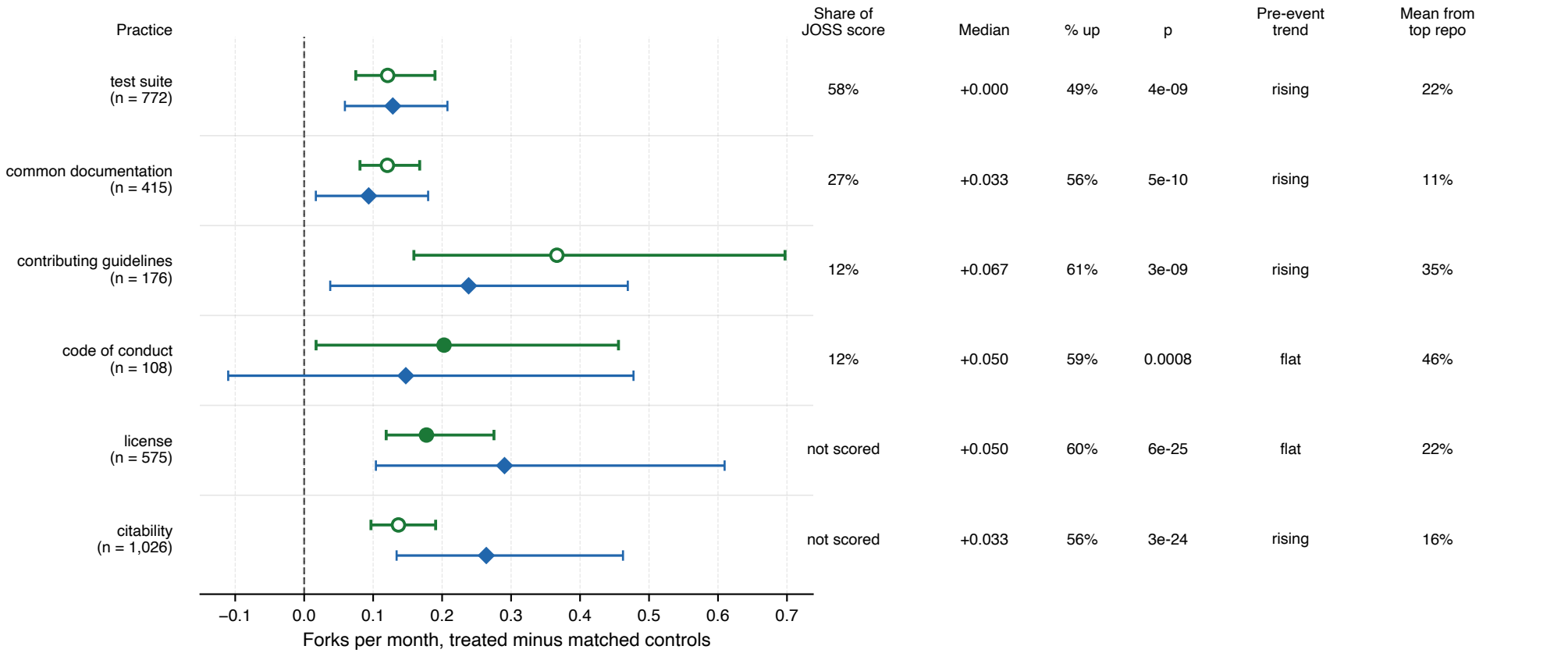
b Fork accrual after adopting a practice, against matched controls
