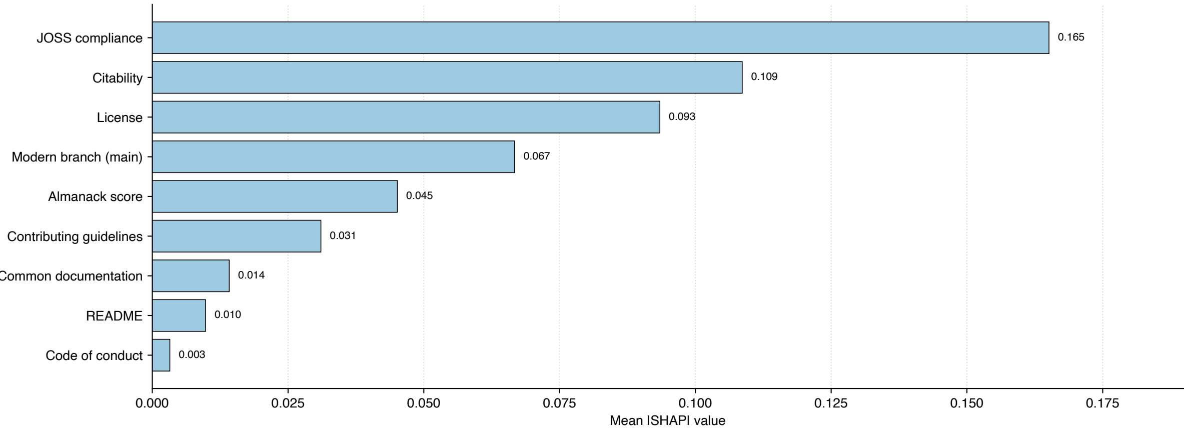
a Sustainability-only model (with JOSS)
