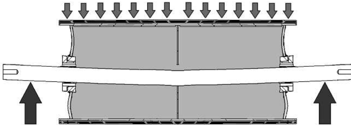
Excessive shaft deflection occurring as a result of an undersized shaft (exaggerated for effect).
