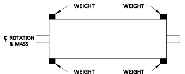
Figure 20 – Dynamically balanced pulley Mass centerline and rotational centerline are on a common axis.
