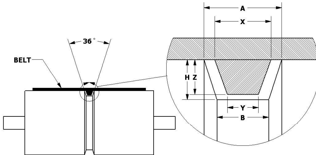
V-Groove Dimensioning
