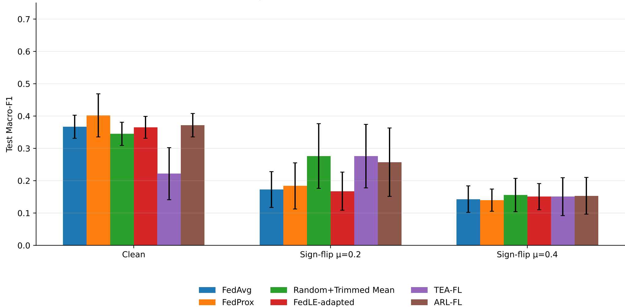
CICIoT2023 performance at \alpha=0.1 (mean \pm SD, n=5)
