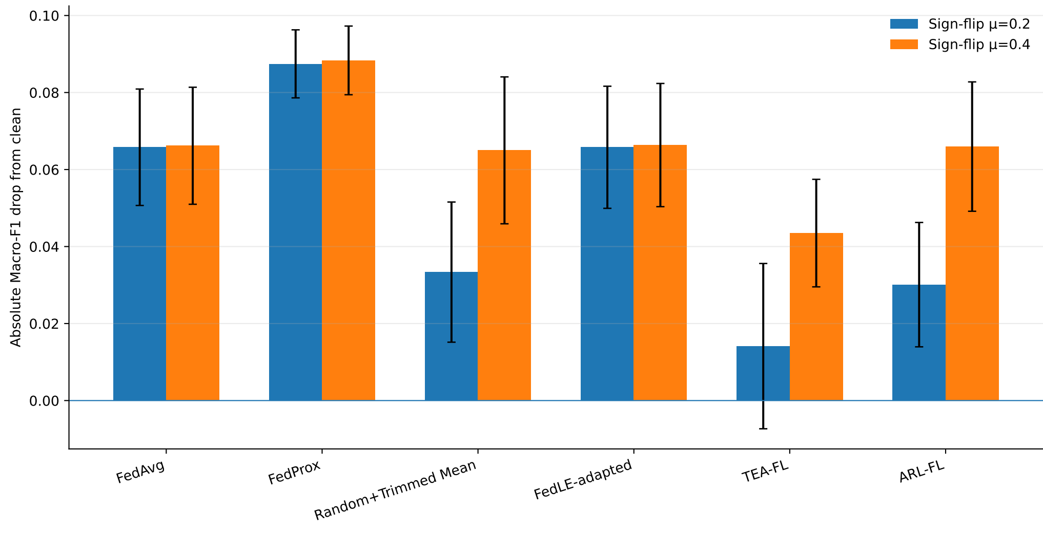
Robustness loss at \alpha=1.0 (mean \pm SD, n=5)
