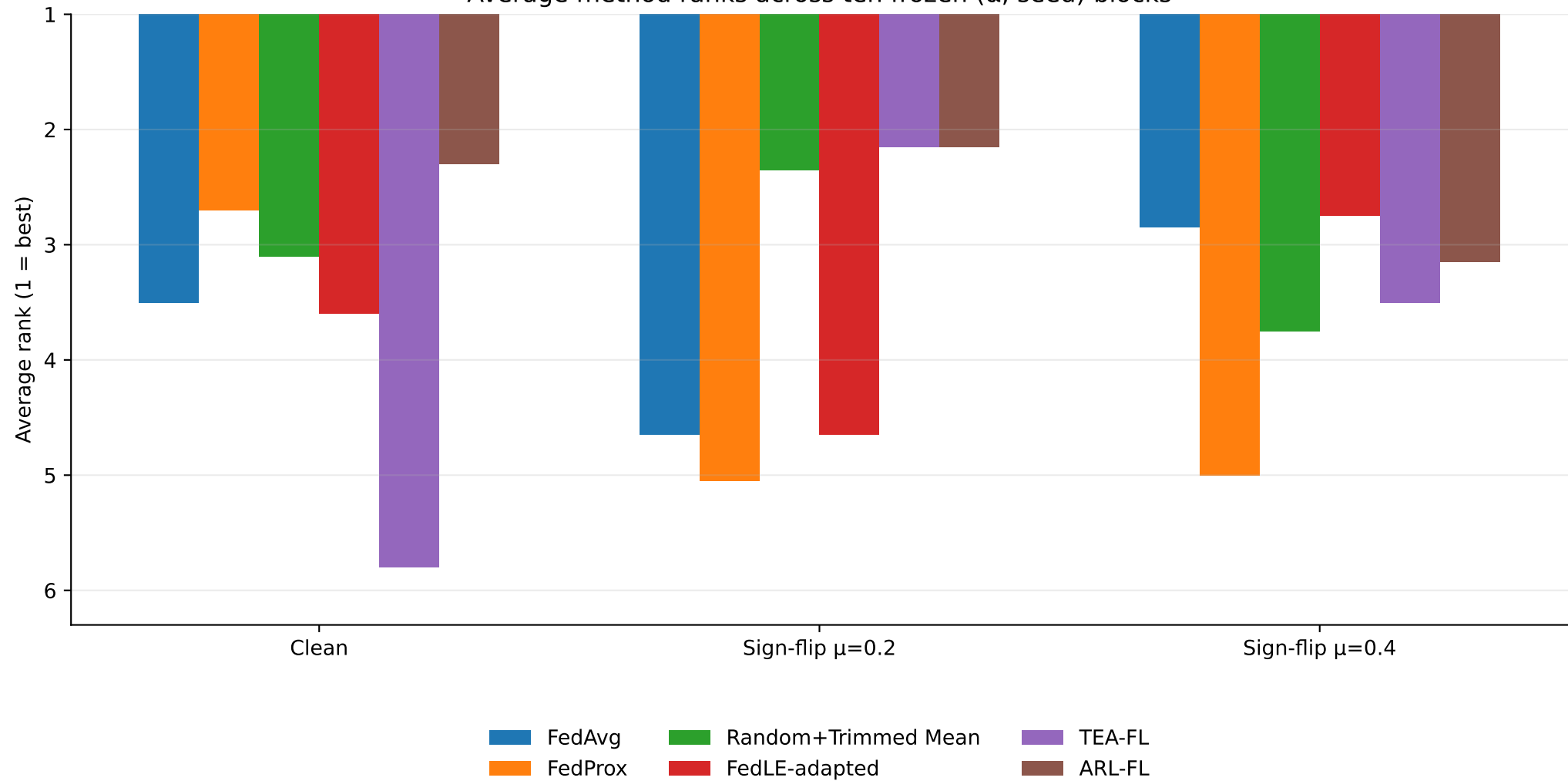
Average method ranks across ten frozen ( \alpha , seed) blocks
