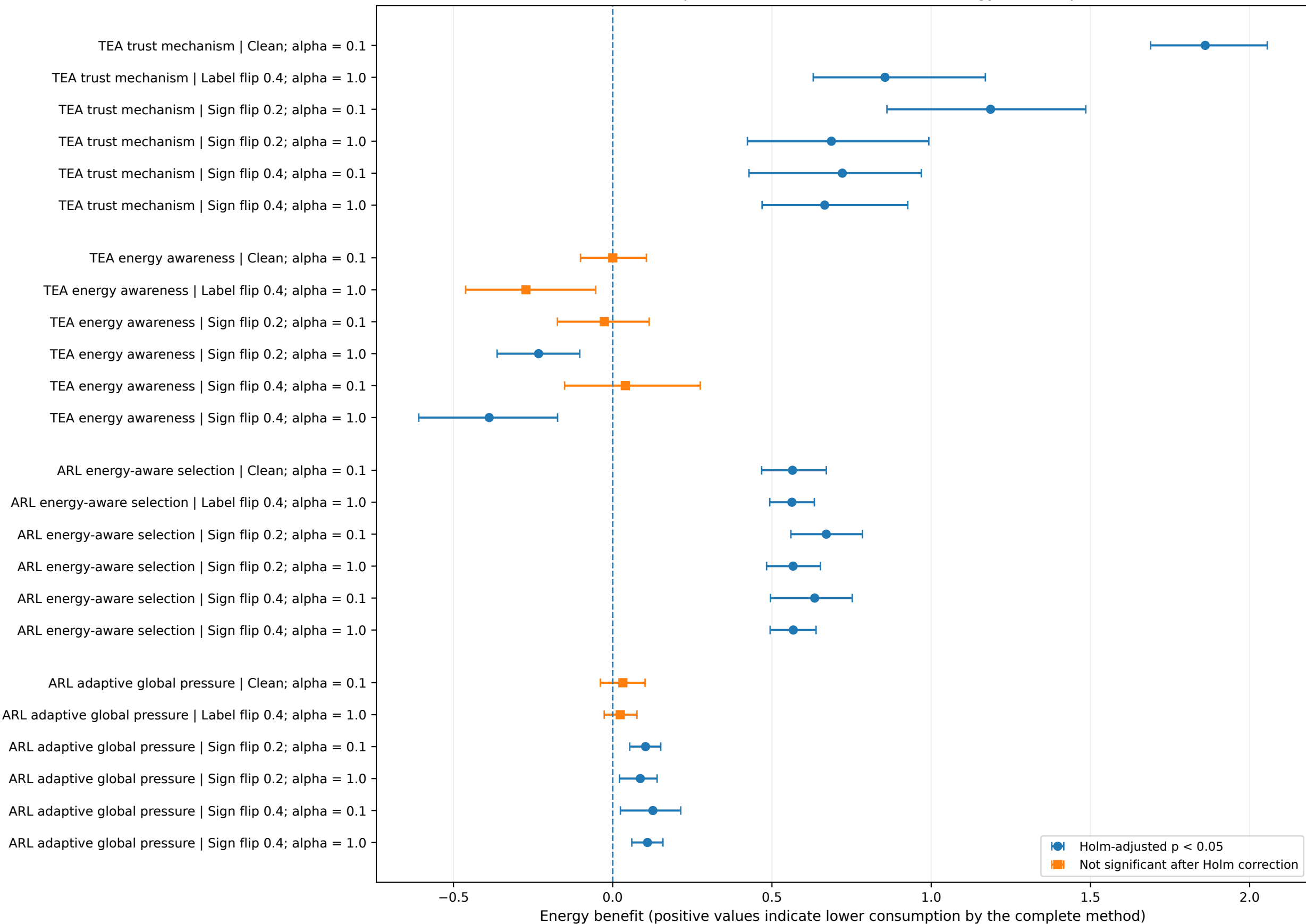
PAMAP2 component effects on normalized energy consumption
