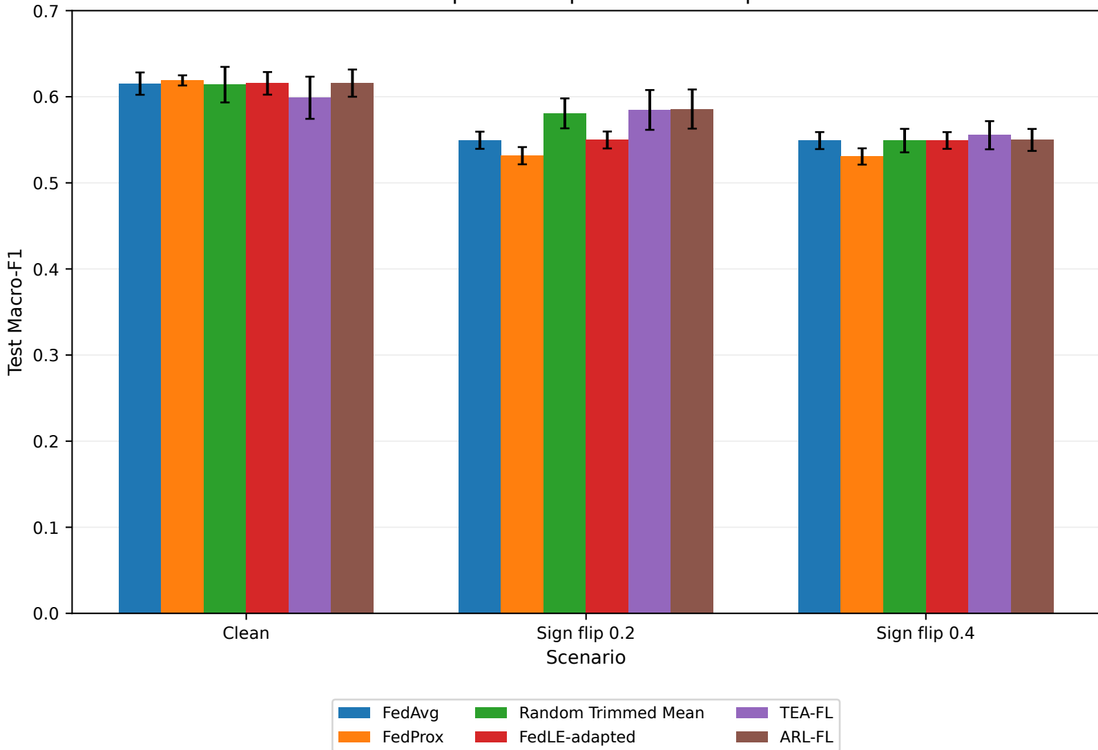
CICIoT2023 predictive performance: \alpha = 1.0
