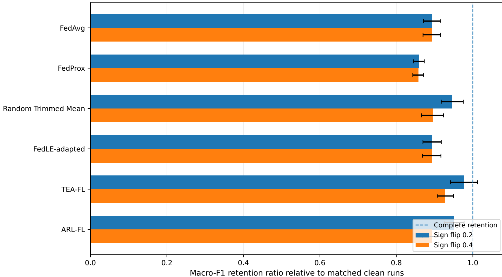
CICIoT2023 robustness retention: \alpha = 1.0
