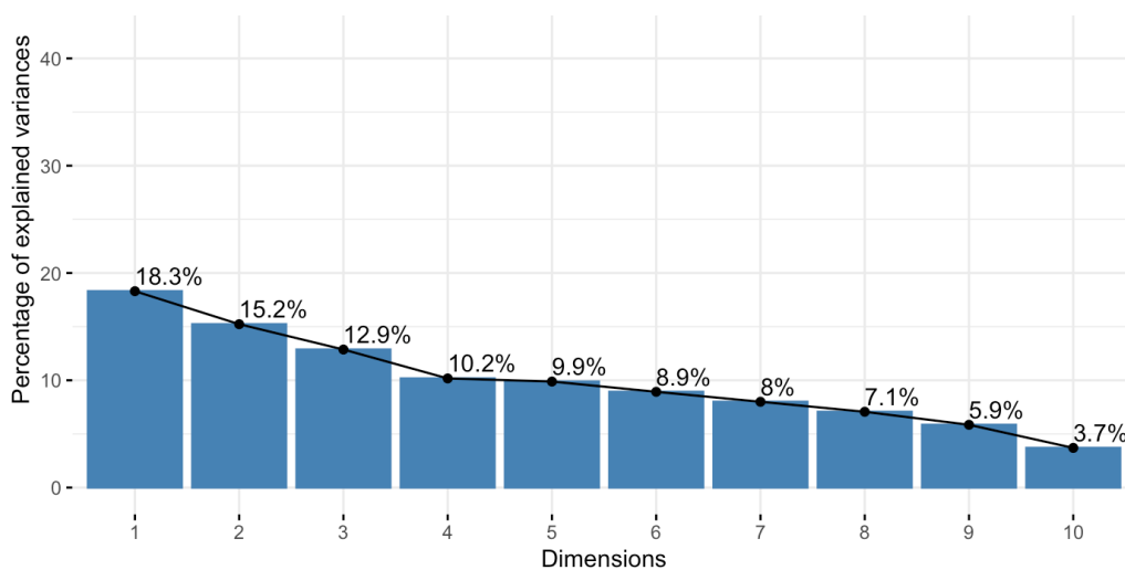
Figure 4. Distribution of Explained Variance Across MCA Dimensions
