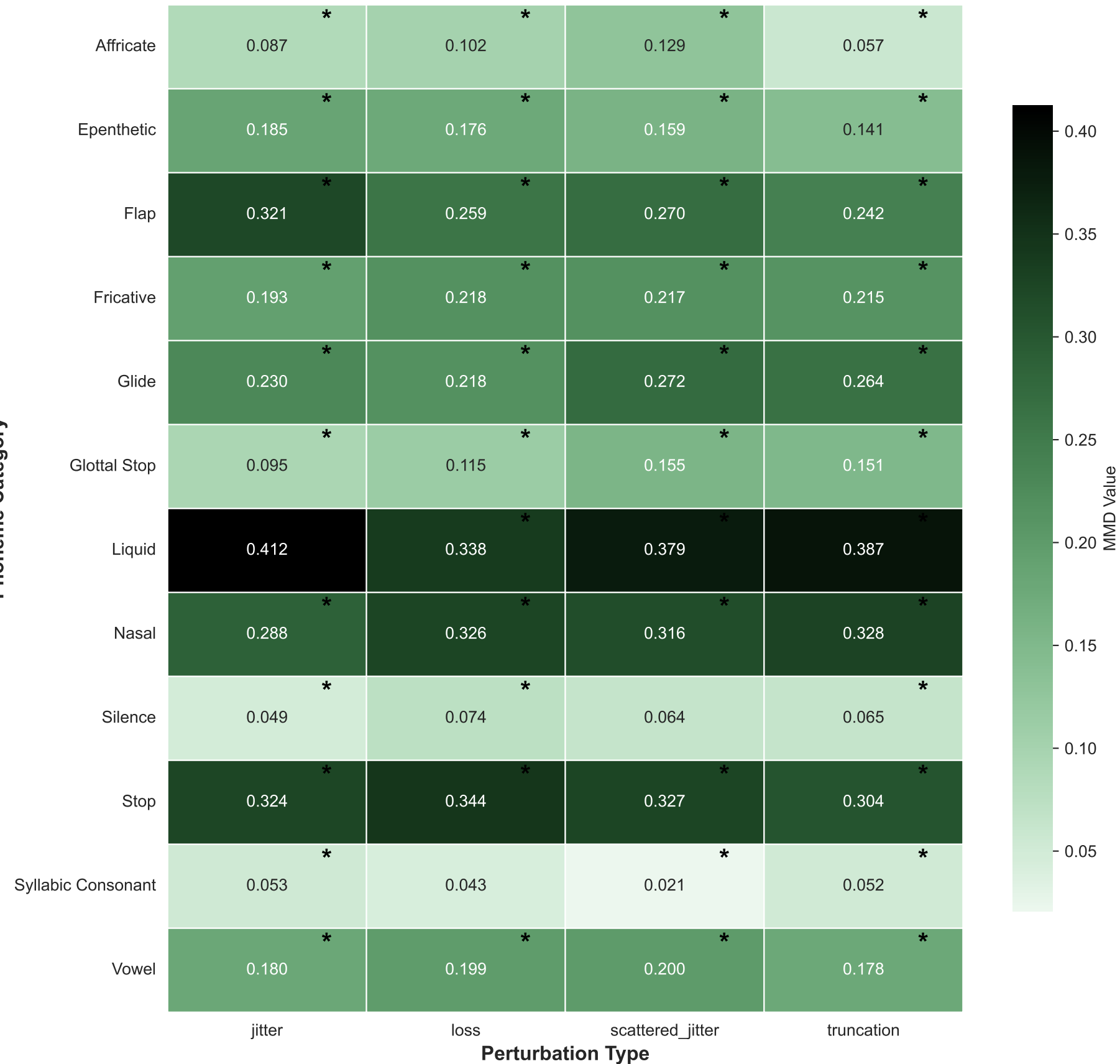
Maximum Mean Discrepancy (MMD)
