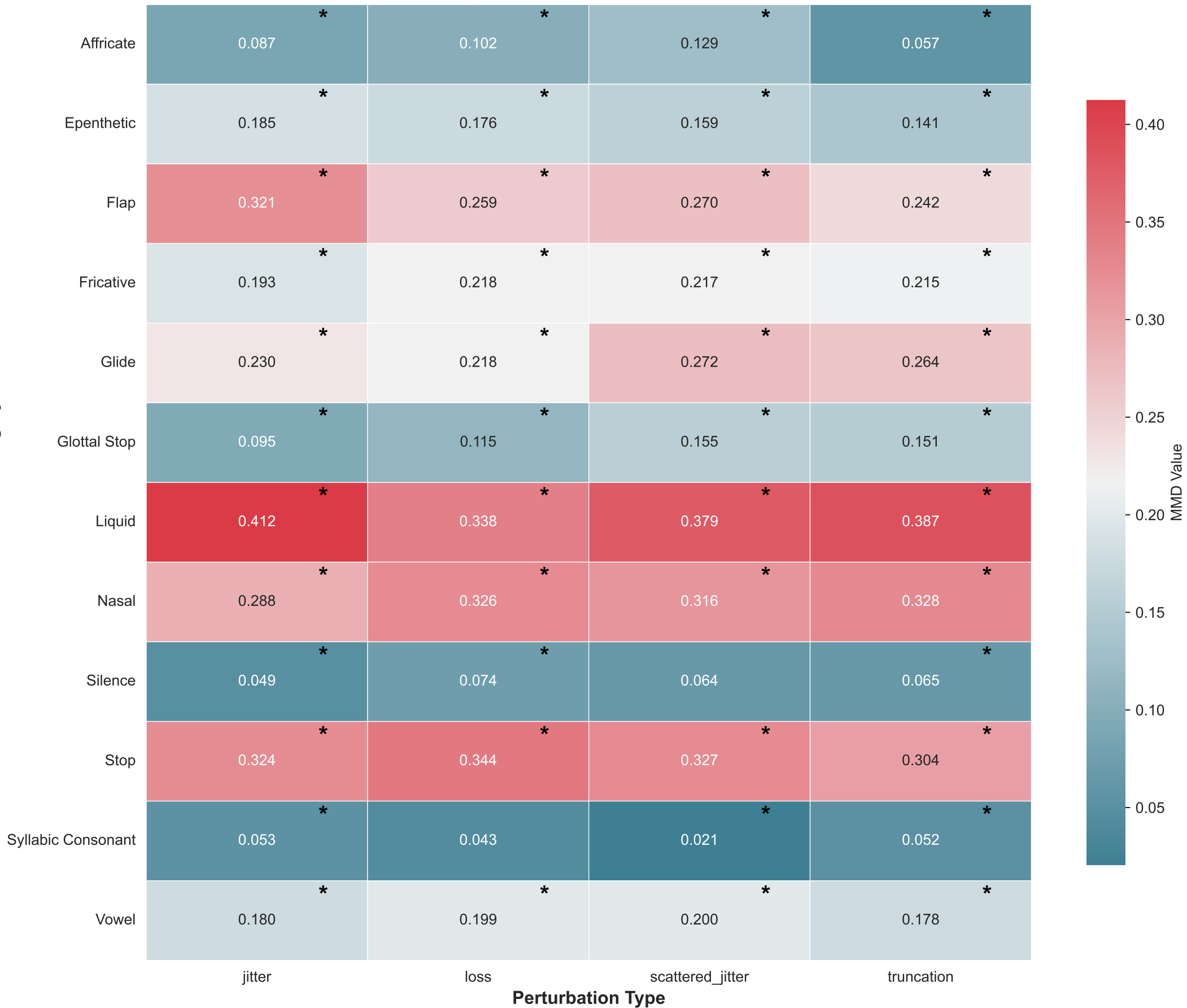
Maximum Mean Discrepancy (MMD) by Phoneme Category and Perturbation Type
