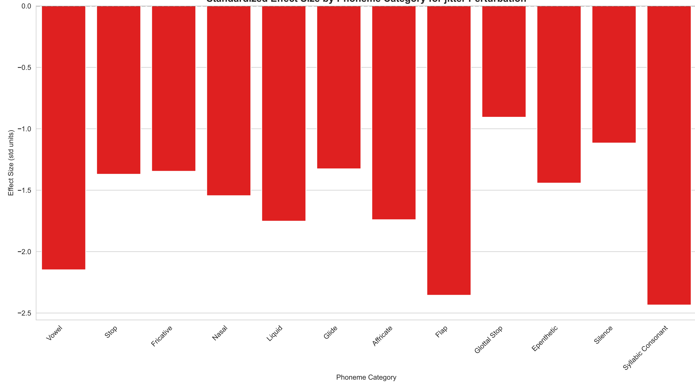
Standardized Effect Size by Phoneme Category for jitter Perturbation
