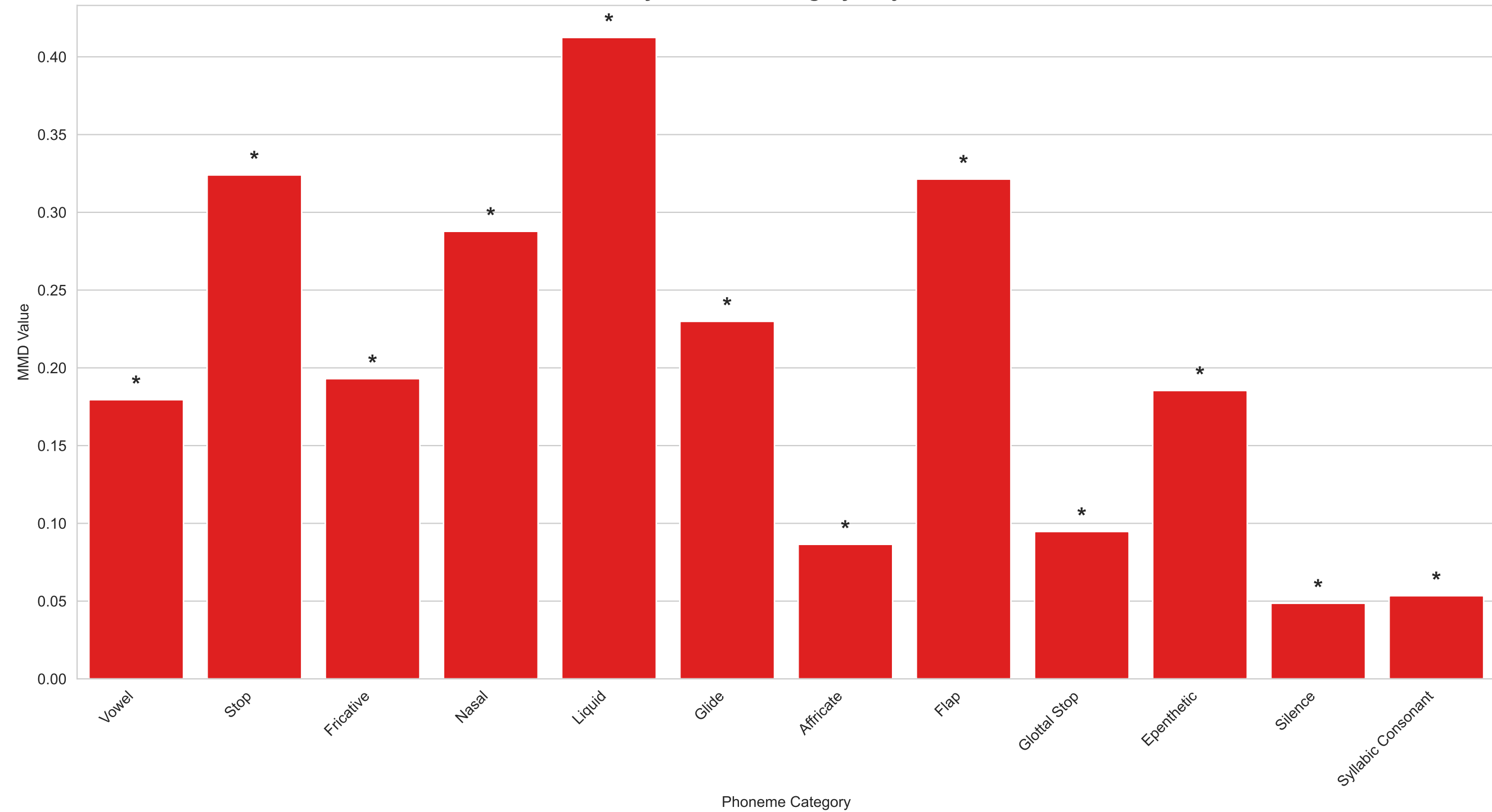
MMD Values by Phoneme Category for jitter Perturbation
