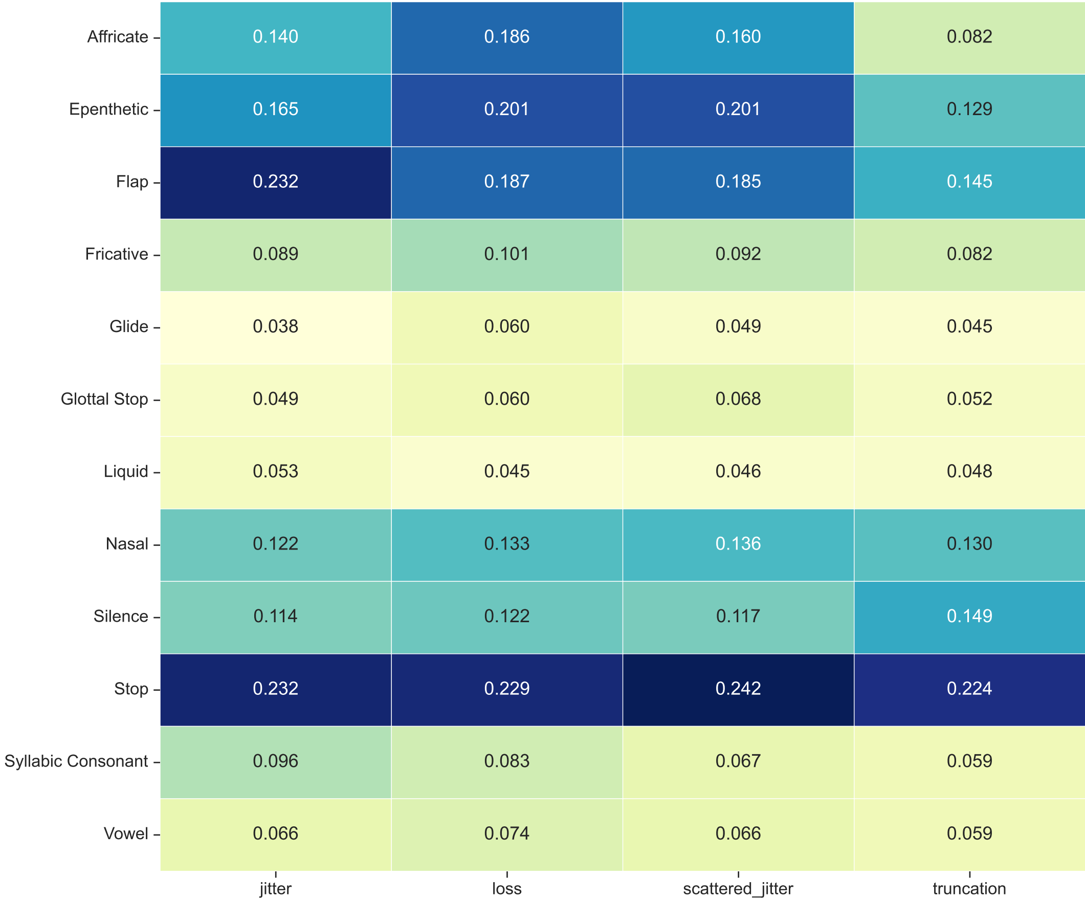
Mean F1 Distances by Category and Perturbation Type (Interaction p=0.0000, significant)
