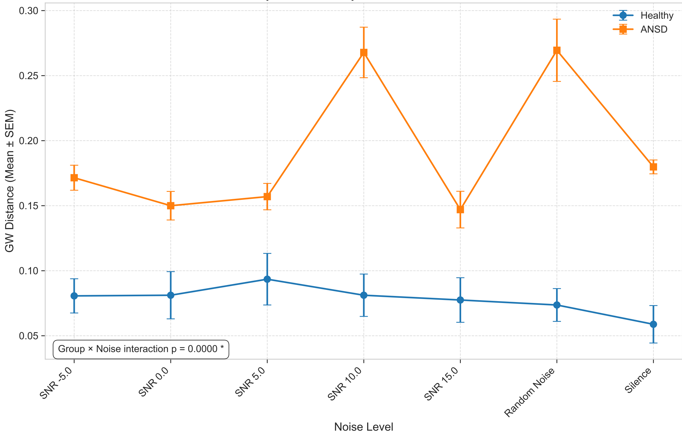
Epenthetic Response to Noise - F3
