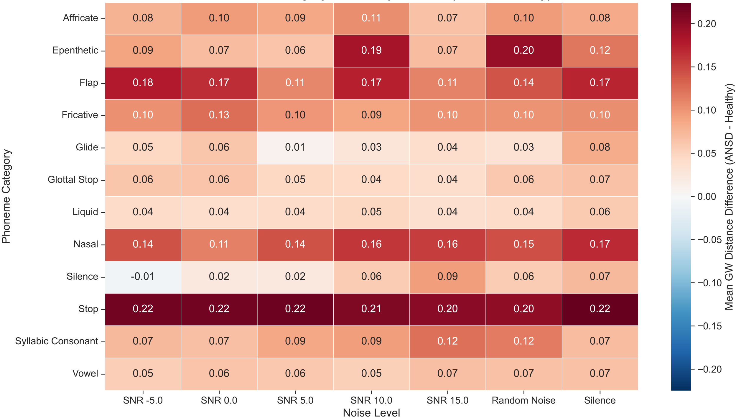
F3: Phoneme Category Sensitivity to Noise (ANSD - Healthy)
