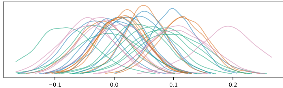
Lagged y Effects
