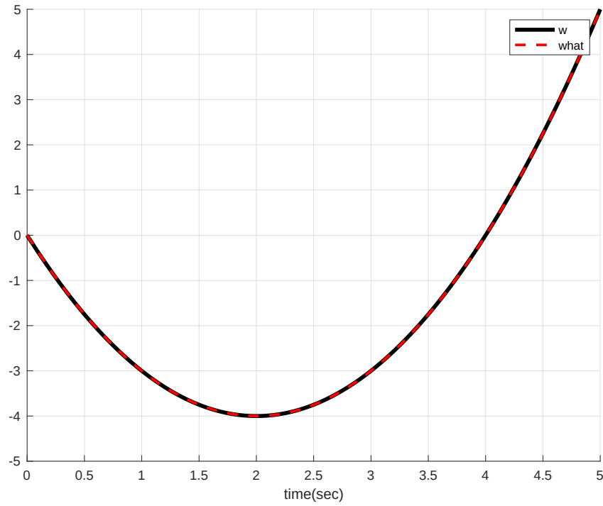
Fig. 4 Disturbance recovered by projection filtering versus actual disturbance
