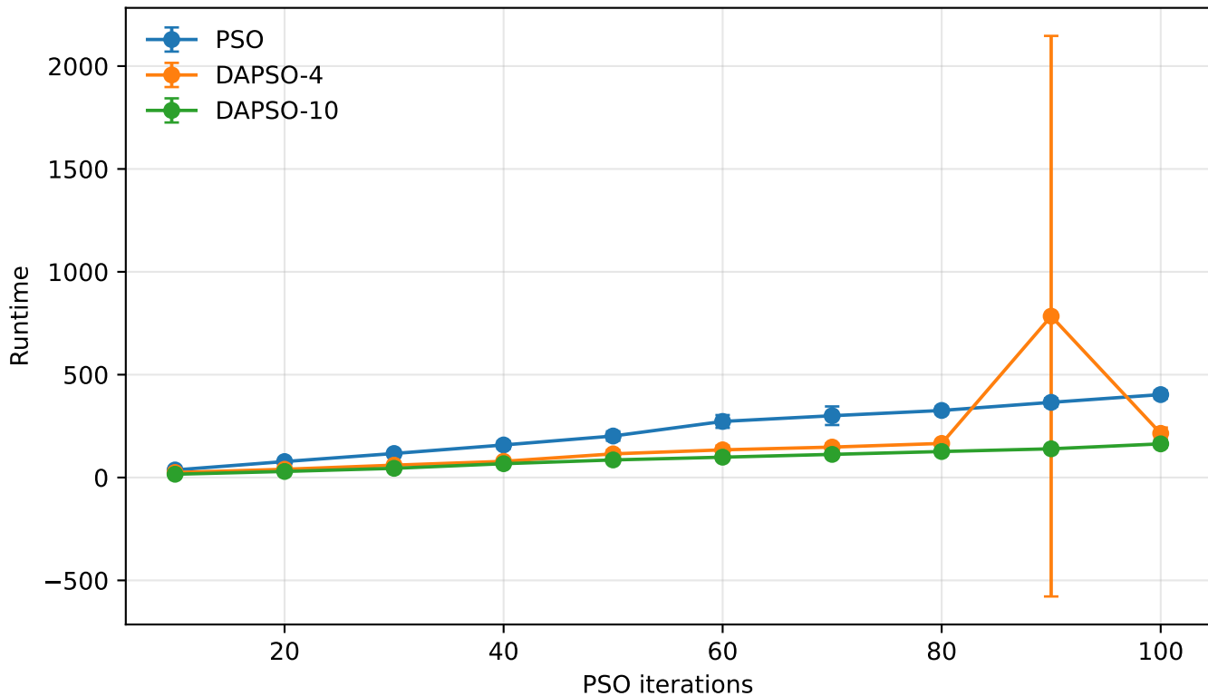
Classification runtime over ten executions
