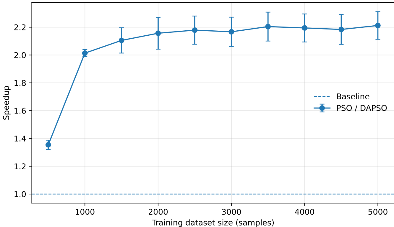
DAPSO speedup with increasing dataset size
