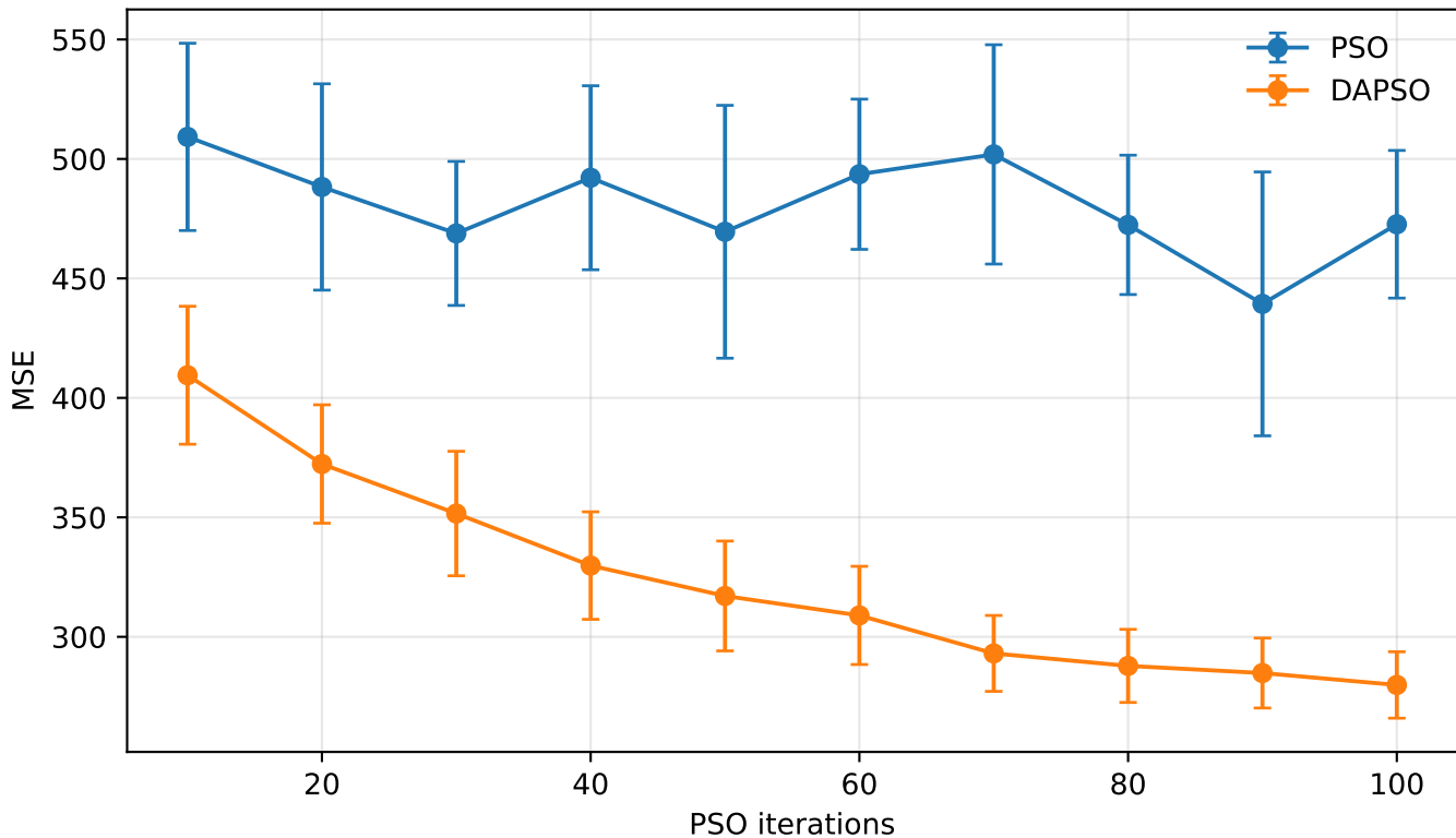
Regression MSE over repeated executions
