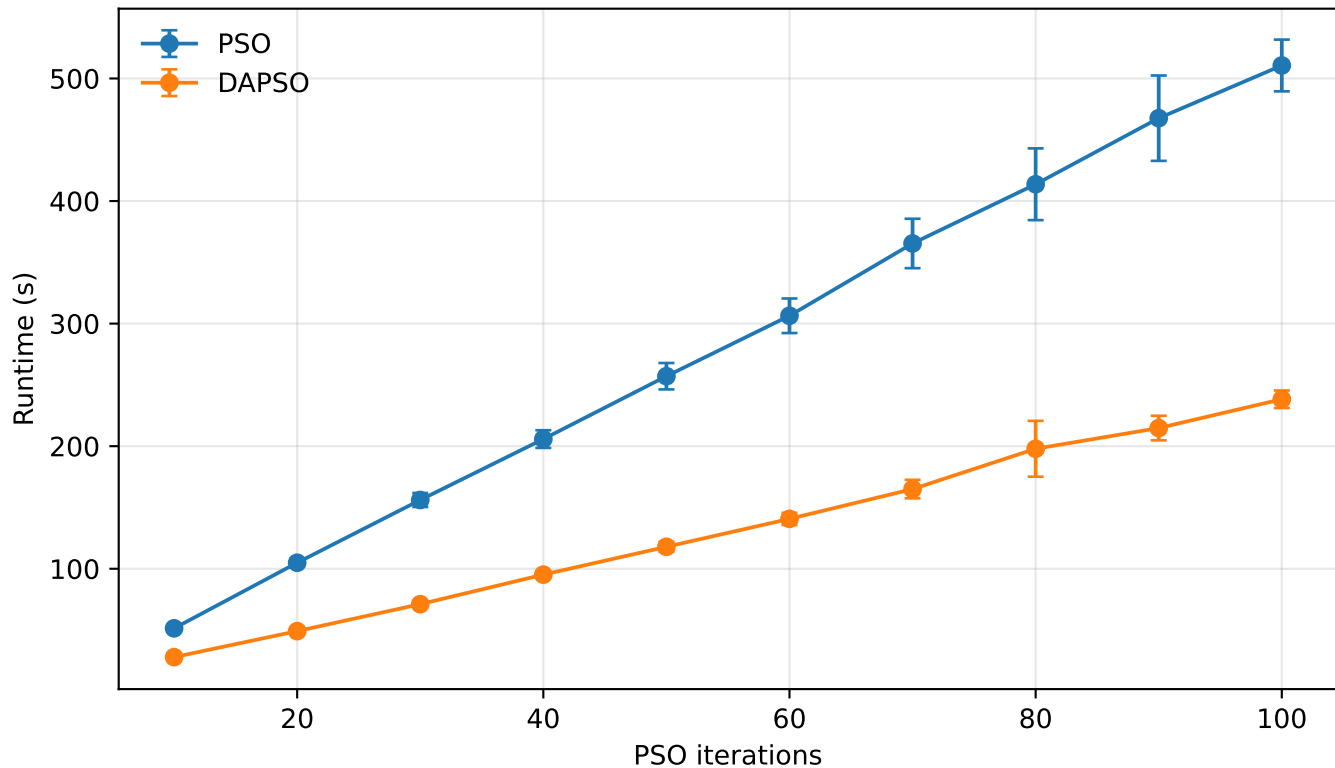
Regression runtime over repeated executions
