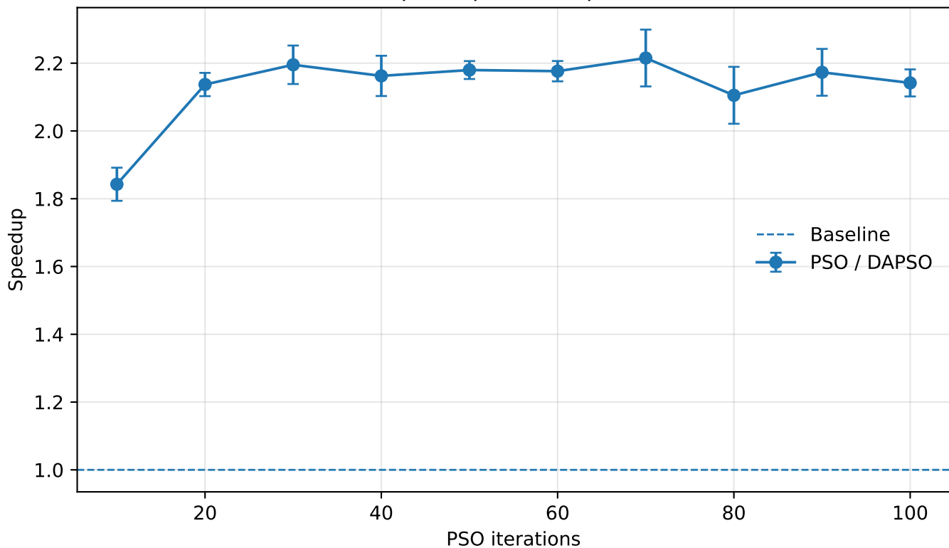
DAPSO speedup over sequential PSO
