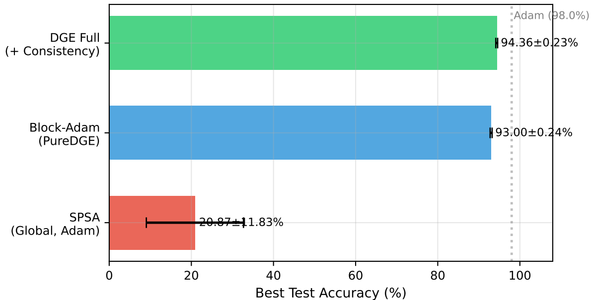
Ablation: Contribution of Each Component (Full MNIST)
