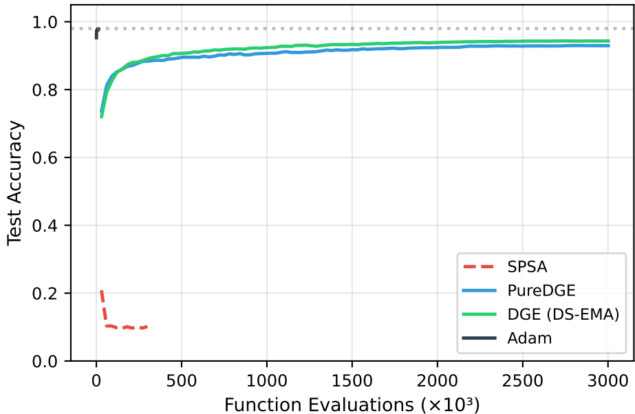
Convergence on MNIST (60K samples)
