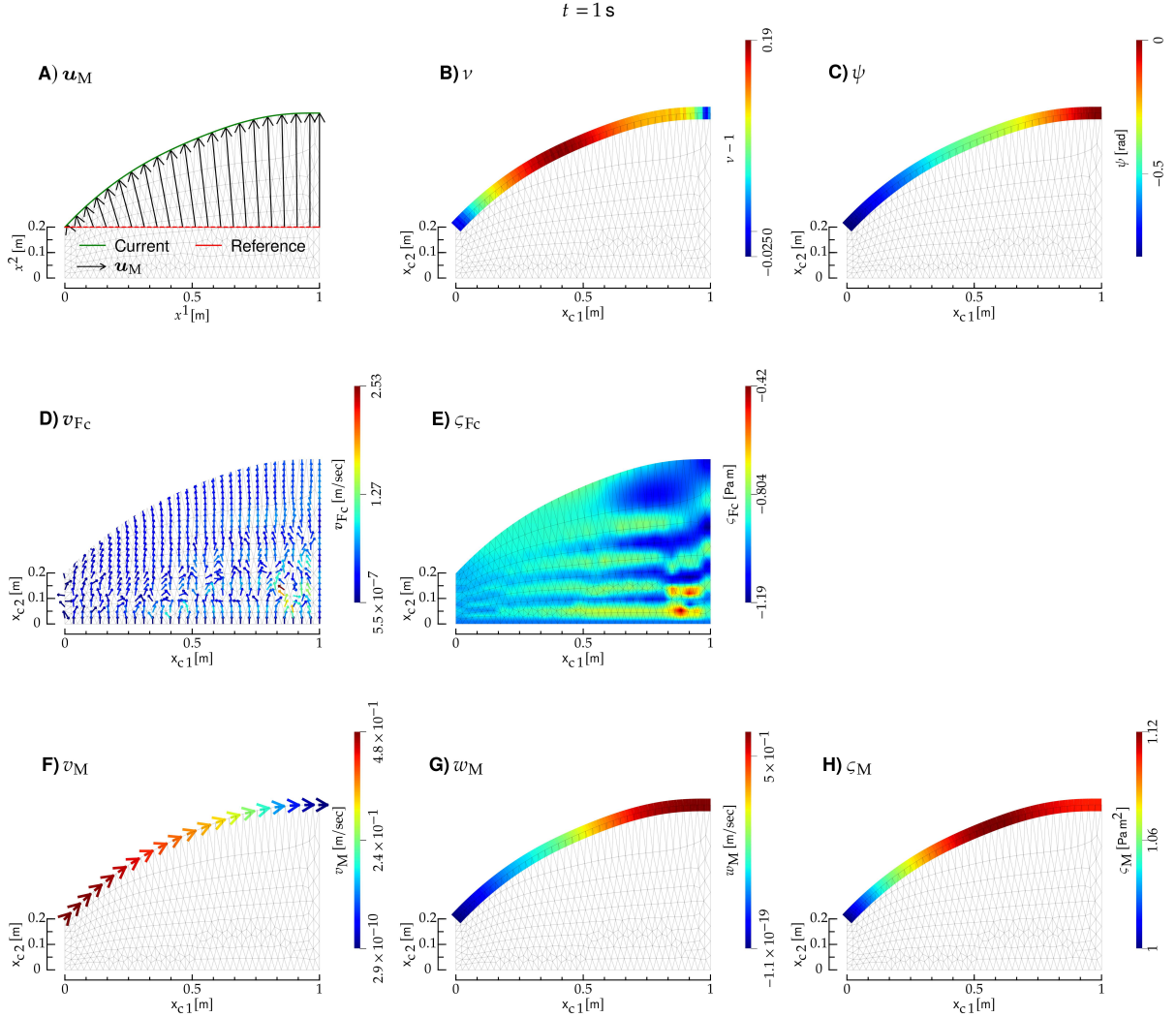
FIG. 6: Interaction between a bulk fluid (F) and a Helfrich membrane (M). Here, F is air, and M an elastomer, and the F Reynolds number is R \sim 200 . A) Reference (r) and current (c) configuration of M (red and green curve, respectively), and M displacement field \mathbf{u}_M (black arrows). B) Stretch field of M. C) Tangent angle of M. D) and E): F velocity and tension, respectively; the notation is the same as in Fig. 2. F) , G) and H): Tangential velocity, normal velocity and tension of M, respectively. All panels refer to the same instant of time, shown on top, and they display also the deformed mesh (gray lines).
