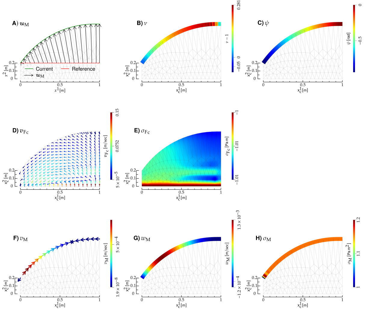
FIG. 7: Interaction between a Bulk fluid (F) and a Helfrich membrane (M). A) Reference (r) and current (c) configuration of M (red and green curve, respectively), and M displacement field \mathbf{u}_M (black arrows). B) Stretch field of M. C) Tangent angle of M. D) and E) : F velocity and tension, respectively; the notation is the same as in Fig. 2. F) , G) and H) : Tangential velocity, normal velocity and tension of M, respectively. All panels refer to the same instant of time, shown on top, and they display also the deformed mesh (gray lines).
