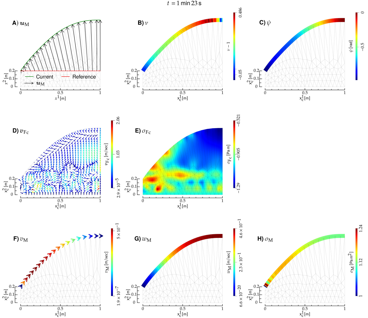
FIG. 6: Interaction between a bulk fluid ( F ) and a Helfrich membrane ( M ). Here, F is air, and M an elastomer, and the F Reynolds number is R \sim 200 . A) Reference ( r ) and current ( c ) configuration of M (red and green curve, respectively), and M displacement field \mathbf{u}_M (black arrows). B) Stretch field of M . C) Tangent angle of M . D) and E) : F velocity and tension, respectively; the notation is the same as in Fig. 2. F) , G) and H) : Tangential velocity, normal velocity and tension of M , respectively. All panels refer to the same instant of time, shown on top, and they display also the deformed mesh (gray lines).
