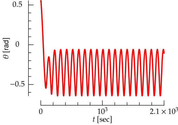
FIG. 8: Angle of the rigid body as a function of time for the interaction between a bulk fluid and a rigid body shown in Fig. 2.
