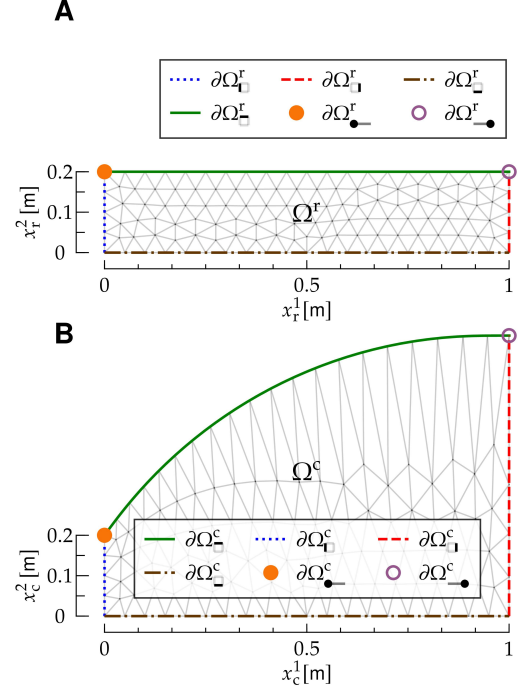
FIG. 5: Reference and current configuration for the interaction between a bulk fluid ( F ) and a Helfrich membrane ( M ). The Figure follows the same notation as Fig. 1, and it represents a vertical channel with mirror symmetry about its mid axis, which coincides with \partial\Omega_{\square}^r ; the right, mirrored part of the channel is not shown. The top edge of the F mesh, \partial\Omega_{\square}^r , coincides with the one-dimensional manifold \Omega_{\square}^r of M .
