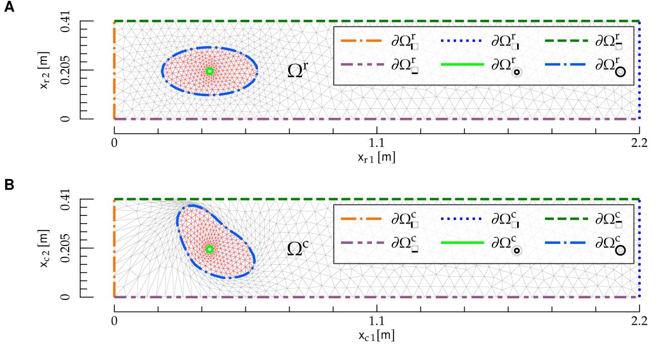
FIG. 3: Reference and current configuration for the interaction between a bulk fluid and an elastic body. The figures follow the same notation as Fig. 1.
