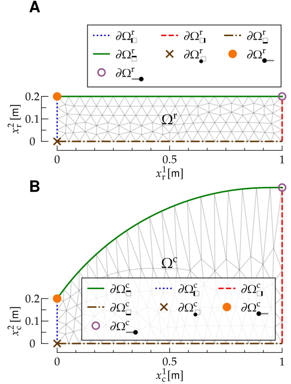
FIG. 5: r and c configuration for the interaction between a bulk fluid ( F ) and a Helfrich membrane ( M ). The Figure follows the same notation as Fig. 1, and it represents a vertical channel with mirror symmetry about its mid axis, which coincides with \partial\Omega_{\square} ; the right, mirrored part of the channel is not shown. The top edge of the F mesh, \partial\Omega_{\square}^r , coincides with the one-dimensional manifold \Omega_{\square}^r of M . The bottom-left point of the F domain \partial\Omega_{\square}^r (brown cross), is marked in both the r and c configuration.
