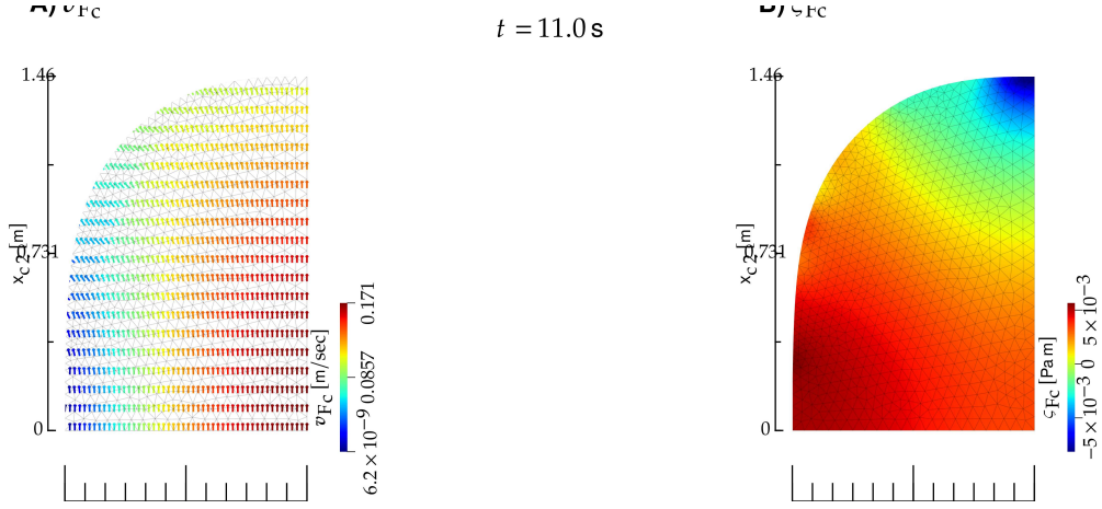
FIG. 7: Interaction between a bulk fluid (F) and a M: F fields. The solution and notation is the same as Fig. 6. A) and B) : F velocity and surface tension, respectively.
