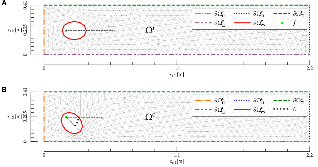
FIG. 1: Reference (r) and current (c) configuration for the interaction between a bulk fluid and a rigid body (R). A) r configuration. The region \Omega^r is given by the rectangle 0 \leq x_{r1} \leq L , 0 \leq x_{r2} \leq h with the elliptical hole (R), and is delimited by the mesh (gray lines). Boundaries in the r configuration are denoted by \partial\Omega_{\Gamma}^r , \partial\Omega_{\Gamma}^r , \partial\Omega_{\Gamma}^r , \partial\Omega_{\Gamma}^r and \partial\Omega_{\Gamma}^r (colored dashed lines). The ellipse focal point f (light green dot) is also shown. B) c configuration. The region \Omega^c is delimited by the mesh (gray lines). Boundaries in the c configuration are denoted by \partial\Omega_{\Gamma}^c , \partial\Omega_{\Gamma}^c , \partial\Omega_{\Gamma}^c , \partial\Omega_{\Gamma}^c and \partial\Omega_{\Gamma}^c (colored dashed lines), and the rotational angle \theta of R is shown as an arc (black dotted line). The Cartesian coordinates \mathbf{x}_c are also shown.
