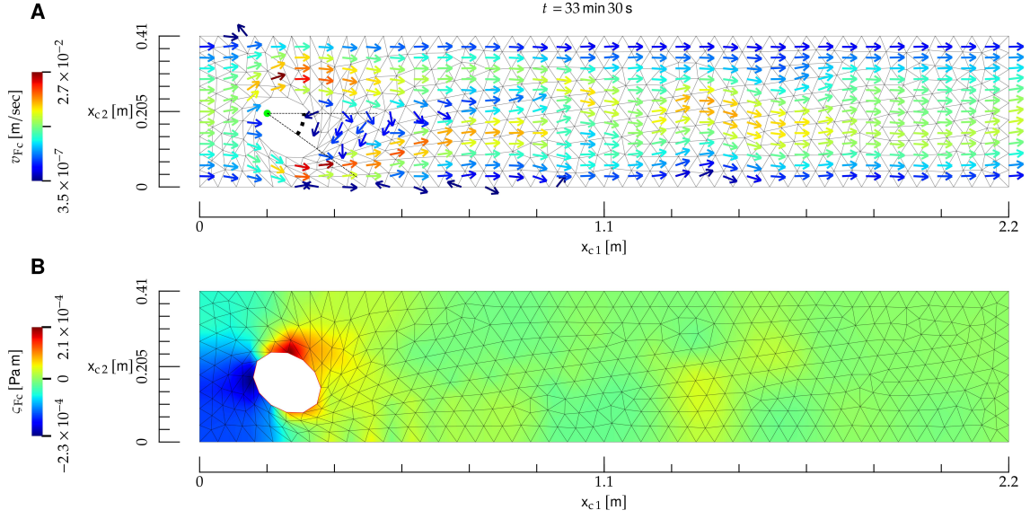
FIG. 1: Interaction between a bulk fluid (F) and a rigid rigid body (R), whose material properties roughly correspond to air (F) and an aerogel (R). A) Temporal snapshot of the mesh (black lines) and velocity field (arrows) at the current time t , shown on top. The direction of the velocity field is indicated by the arrows, and its norm by their color; the direction of arrows with velocity close to zero is not defined. Here, R (ellipse) is allowed to pivot about its left focal point (red dot), and the related angle with respect to the x_{c1} direction is denoted by a black dashed arc. Here, the Reynolds number is R \sim 2 \times 10^2 . B) Color map of the surface tension at the current instant of time t .
