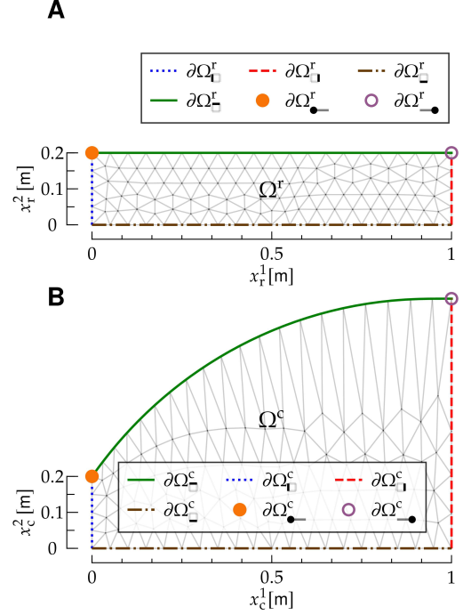
FIG. 5: Reference and current configuration for the interaction between a bulk fluid ( \mathbf{F} ) and a Helfrich membrane ( \mathbf{M} ). The Figure follows the same notation as Fig. 2, and it represents a vertical channel with mirror symmetry about its mid axis, which coincides with \partial\Omega_{\square}^r ; the right, mirrored part of the channel is not shown. The top edge of the \mathbf{F} mesh, \partial\Omega_{\square}^r , coincides with the one-dimensional manifold \Omega_{\square}^r of \mathbf{M} .
