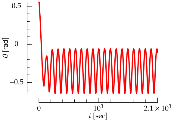
FIG. 3: Angle of the rigid body as a function of time for the interaction between a bulk fluid and a rigid body shown in Fig. 2.
