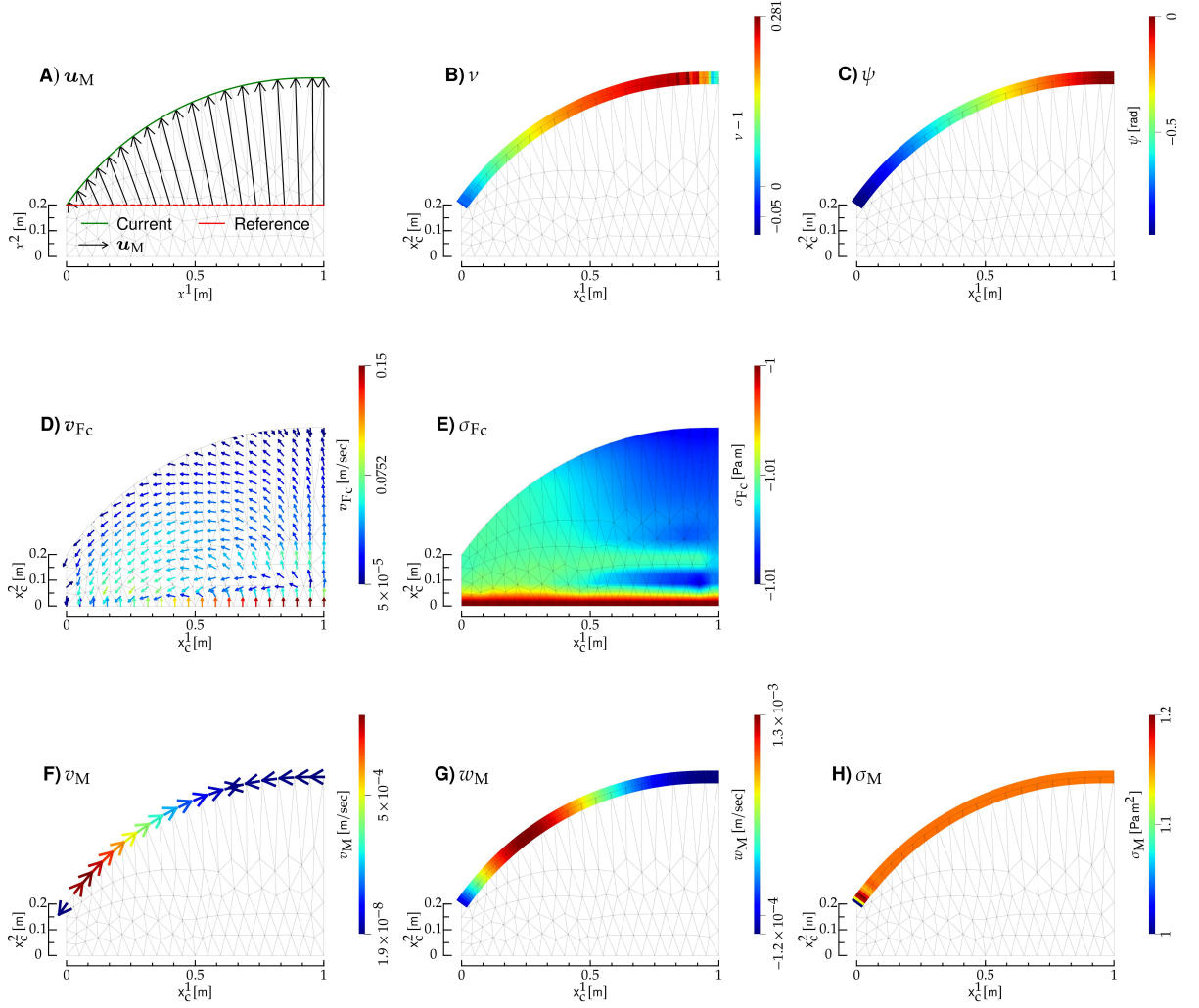
FIG. 7: Interaction between a Bulk fluid (F) and a Helfrich membrane (M) . A) Reference (r) and current (c) configuration of M (red and green curve, respectively), and M displacement field \mathbf{u}_M (black arrows). B) Stretch field of M . C) Tangent angle of M . D) and E) : F velocity and tension, respectively; the notation is the same as in Fig. 2. F) , G) and H) : Tangential velocity, normal velocity and tension of M , respectively. All panels refer to the same instant of time, shown on top, and they display also the deformed mesh (gray lines).
