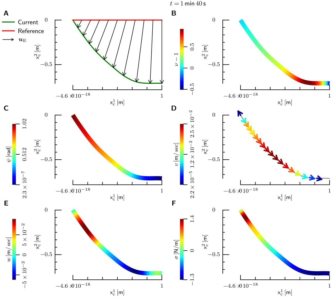
FIG. 7: Helfrich fluid layer described with the generalized arc length gauge. The layer is subjected to a gravitational field directed along the X^2 axis, in the direction of negative X^2 . A) Displacement field \vec{U} , which relates the reference and the current configuration, shown in red and green, respectively. B) Stretching \nu . C) Tangent angle \psi . D) Tangential velocity. Arrows show the velocity direction, and the color code the velocity norm. E) Normal velocity, whose value is shown with the color code. F) Surface tension. All panels refer to the same instant of time, shown on top.
