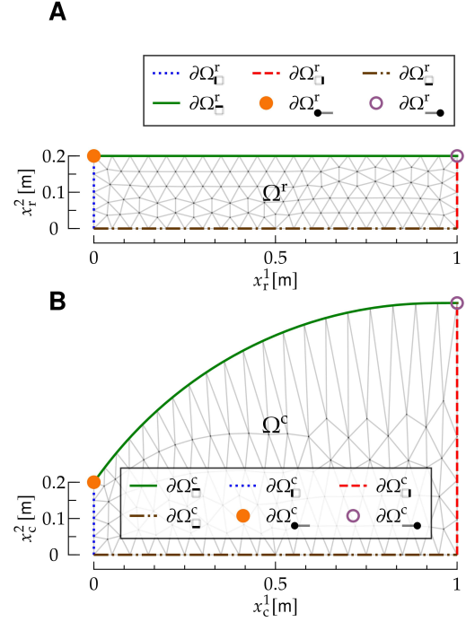
FIG. 6: Reference and current configuration for the interaction between a bulk fluid ( F ) and a Helfrich membrane ( M ). The figure follows the same notation as ???. The top edge of the F mesh, \partial\Omega_{\square}^r , coincides with the one-dimensional manifold \Omega_{\square}^r of M .
