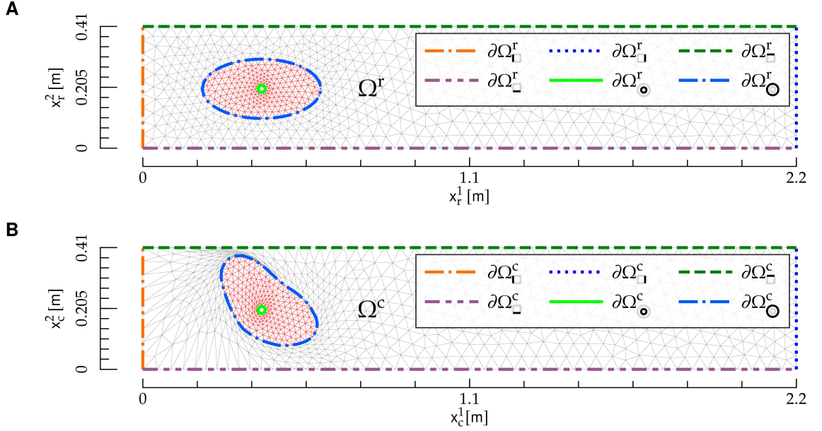
FIG. 4: Reference and current configuration for the interaction between a bulk fluid and an elastic body. The figures follows the same notation as ??.
