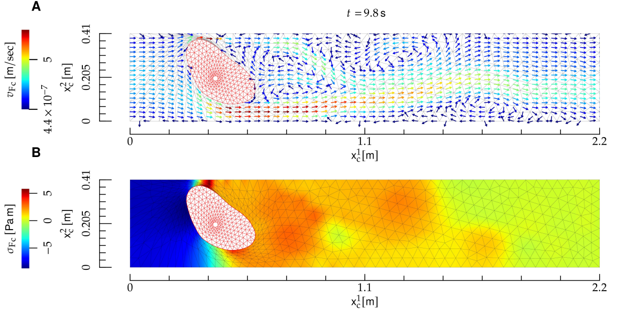
FIG. 5: Interaction between a bulk fluid and an elastic body (E) (a hydrogel). The notation is the same as in ??, and the elastic body is depicted as a red mesh. Here, the Reynolds number is R \sim 2 \times 10^2 . The E deformation is not symmetric under the mirror symmetry x_c^2 \rightarrow h - x_c^2 , where h is the height of the F domain, because the center of E is not located at x_c^2 = h/2 .
