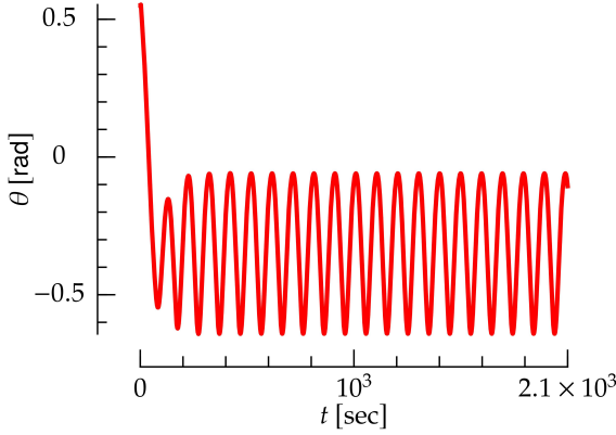
FIG. 3: Angle of the rigid body as a function of time for the interaction between a bulk fluid and a rigid body shown in ??.
