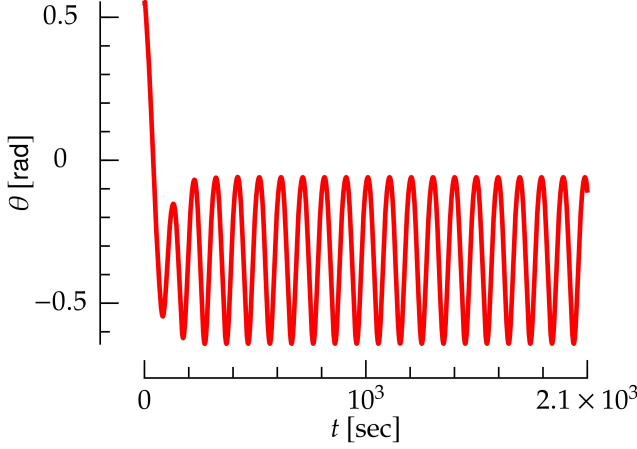
FIG. A.1: Angle of the red body as a function of time for the interaction between a bulk fluid and a red body shown in ??.
