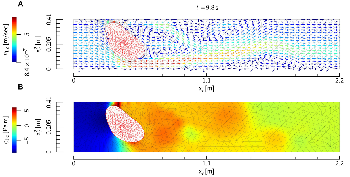
FIG. 5: Interaction between a bulk fluid and an elastic body ( E ) (a hydrogel). The notation is the same as in Fig. 3, and the elastic body is depicted as a red mesh. Here, the Reynolds number is R \sim 2 \times 10^2 . The E deformation is not symmetric under the mirror symmetry x_c^2 \rightarrow h - x_c^2 , where h is the height of the F domain, because the center of E is not located at x_c^2 = h/2 .
