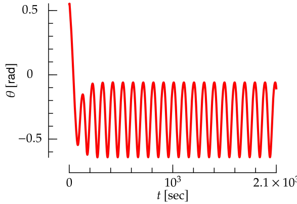
FIG. 3: Angle of the body as a function of time for the interaction between a bulk fluid and a rigid body shown in Fig. 2.
