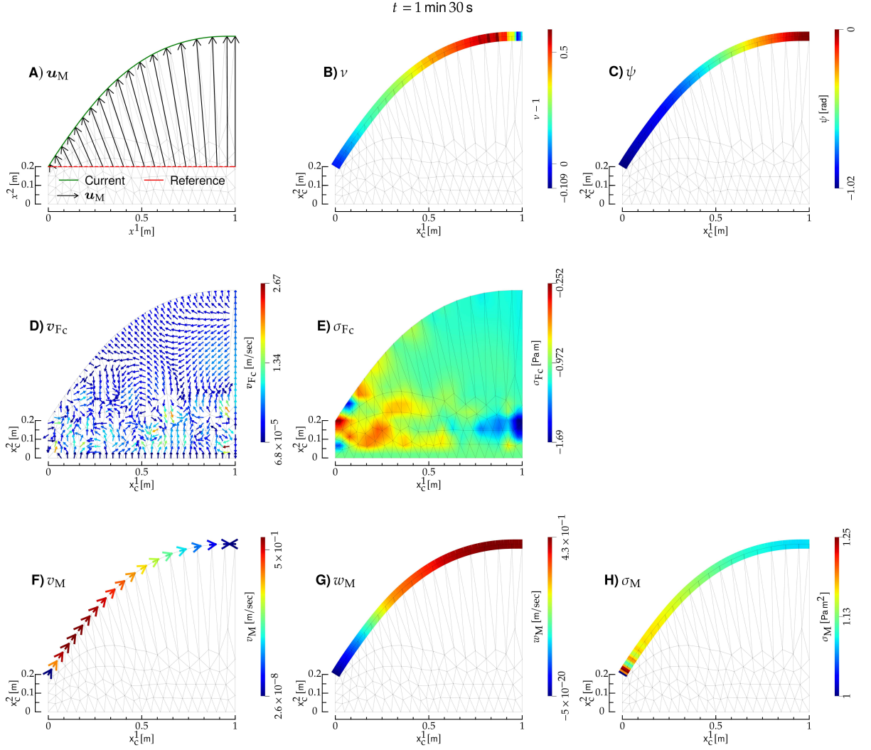
FIG. 7: Interaction between a bulk fluid (F) and a Helfrich membrane (M). Here, F is air, and M an elastomer. A) Reference (r) and current (c) configuration of M (red and green curve, respectively), and M displacement field \mathbf{u}_M (black arrows). B) Stretch field of M . C) Tangent angle of M . D) and E) : F velocity and tension, respectively; the notation is the same as in Fig. 2. F) , G) and H) : Tangential velocity, normal velocity and tension of M , respectively. All panels refer to the same instant of time, shown on top, and they display also the deformed mesh (gray lines).
