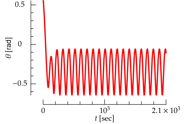
FIG. 8: Angle of the rigid body as a function of time for the interaction between a bulk fluid and a rigid body shown in Fig. 2.
