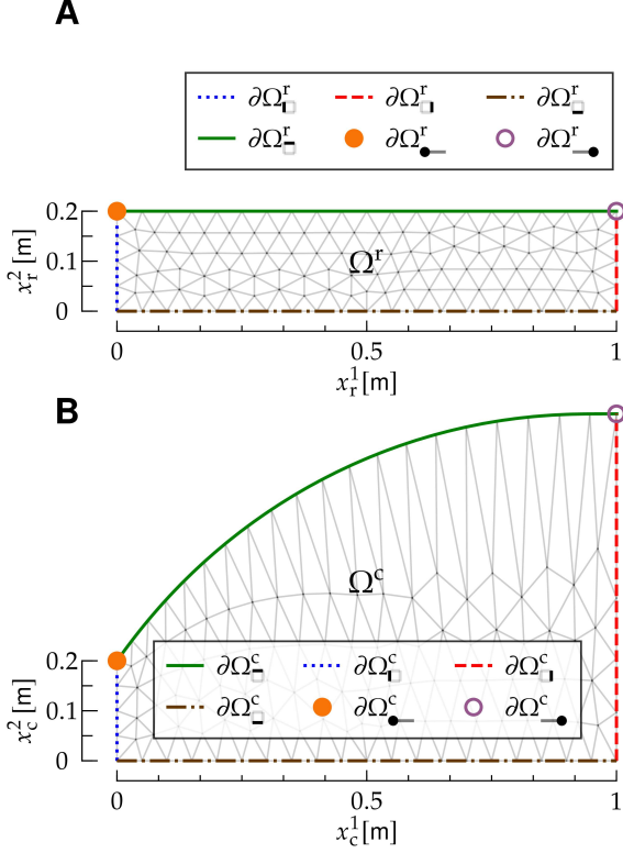
FIG. 5: Reference and current configuration for the interaction between a bulk fluid (F) and a Helfrich membrane (M). The Figure follows the same notation as Fig. 1, and it represents a vertical channel with mirror symmetry about its mid axis, which coincides with \partial\Omega_{\square} ; the right, mirrored part of the channel is not shown. The top edge of the F mesh, \partial\Omega_{\square}^r , coincides with the one-dimensional manifold \Omega_{\square}^r of M.
