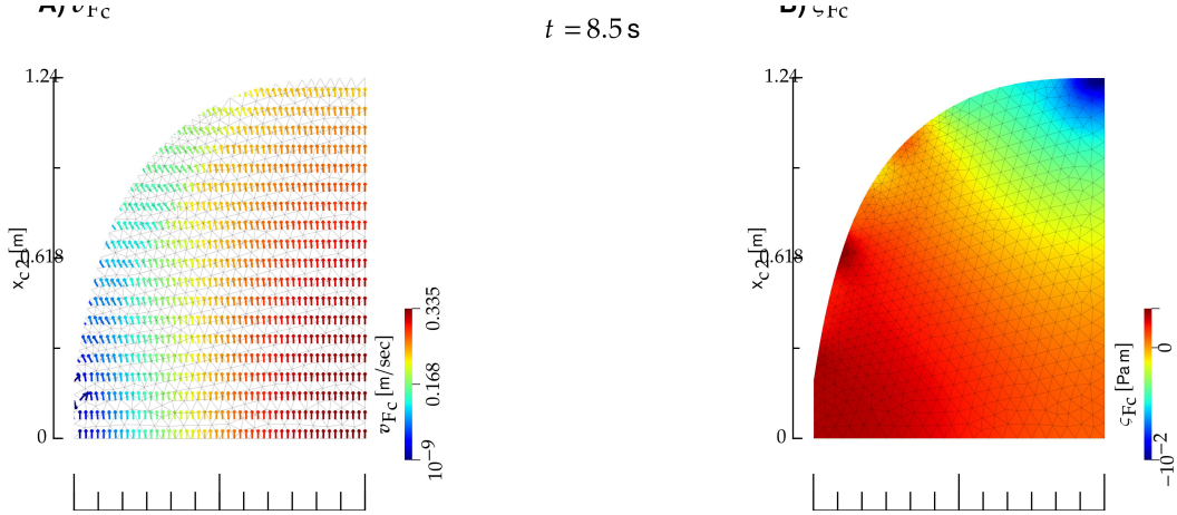
FIG. 7: Interaction between a bulk fluid (F) and a M : F fields. The solution and notation is the same as Fig. 6. A) and B) : F velocity and surface tension, respectively.
