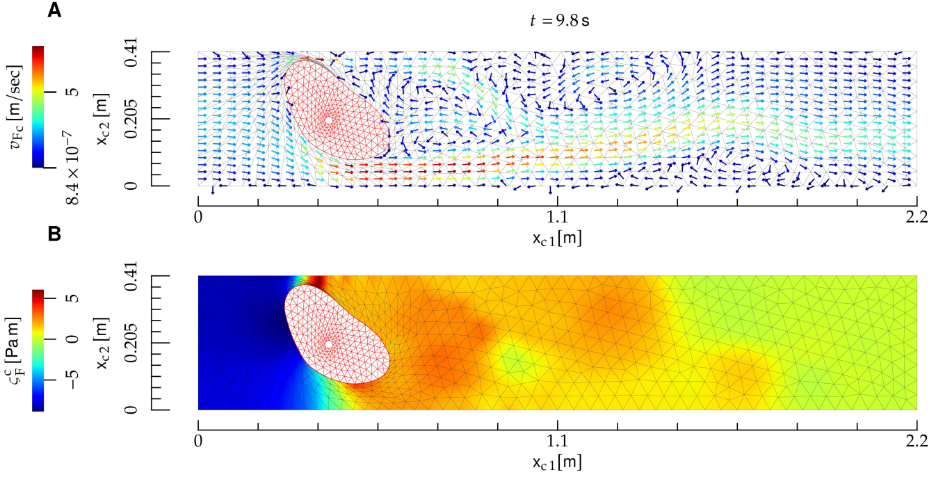
FIG. 4: Interaction between a bulk fluid and an elastic body (E) (a hydrogel). The notation is the same as in Fig. 2, and the elastic body is depicted as a red mesh. Here, the Reynolds number is R \sim 2 \times 10^2 . The E deformation is not symmetric under the mirror symmetry x_{c2} \rightarrow h - x_{c2} , where h is the height of the F domain, because the center of E is not located at x_{c2} = h/2 .
