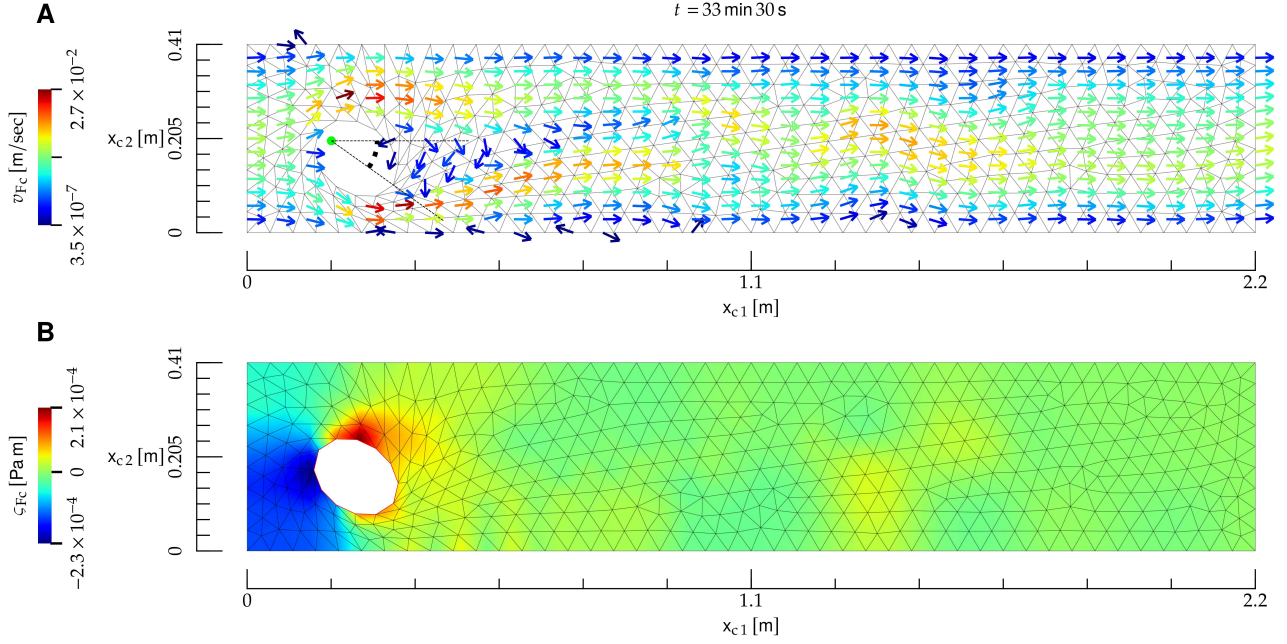
FIG. 2: Interaction between a bulk fluid (F) and a rigid rigid body (R), whose material properties roughly correspond to air (F) and an aerogel (R). A) Temporal snapshot of the mesh (black lines) and velocity field (arrows) at the current time t , shown on top. The direction of the velocity field is indicated by the arrows, and its norm by their color; the direction of arrows with velocity close to zero is not defined. Here, R (ellipse) is allowed to pivot about its left focal point (red dot), and the related angle with respect to the x_{c1} direction is denoted by a black dashed arc. Here, the Reynolds number is R \sim 2 \times 10^2 . B) Color map of the surface tension at the current instant of time t .
