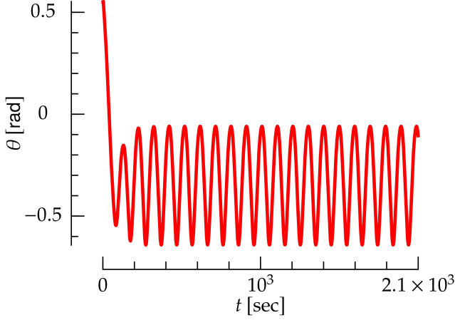
FIG. A.1: Angle of the red body as a function of time for the interaction between a bulk fluid and a rigid body shown in ??.
