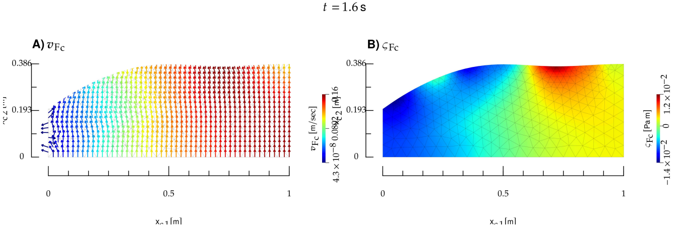
FIG. 7: Interaction between a bulk fluid ( F ) and a M : F fields. The solution and notation is the same as Fig. 6. A ) and B ): F velocity and surface tension, respectively.
