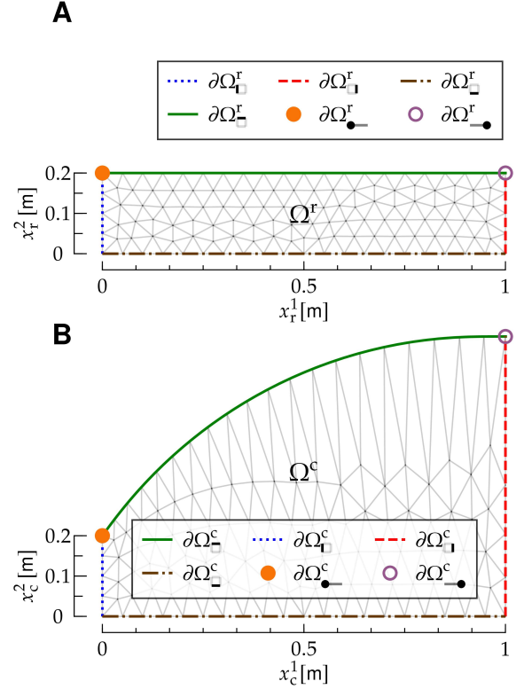
FIG. 5: Reference and current configuration for the interaction between a bulk fluid ( F ) and a Helfrich membrane ( M ). The Figure follows the same notation as Fig. 1, and it represents a vertical channel with mirror symmetry about its mid axis, which coincides with \partial\Omega_{\square} ; the right, mirrored part of the channel is not shown. The top edge of the F mesh, \partial\Omega_{\square}^r , coincides with the one-dimensional manifold \Omega_{\square}^r of M .
