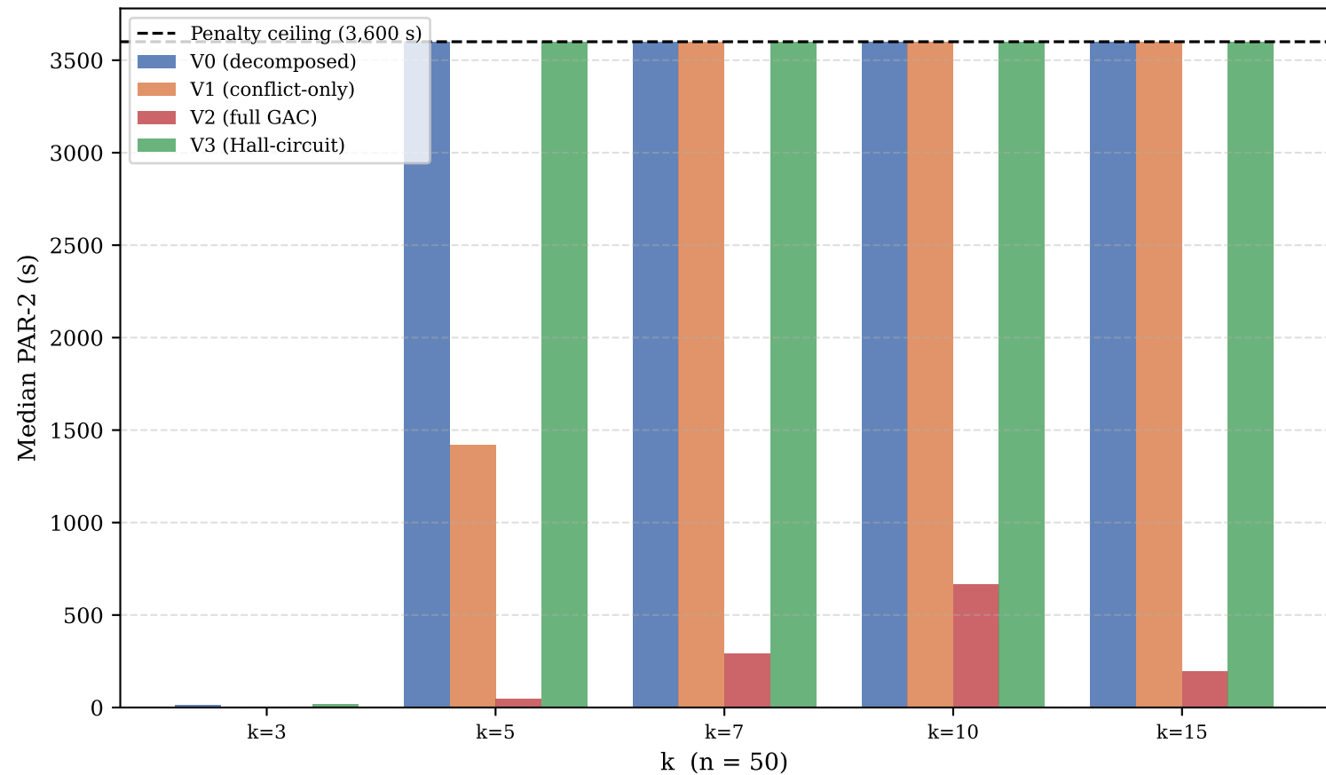
PAR-2 scores at n = 50 (lower is better)
