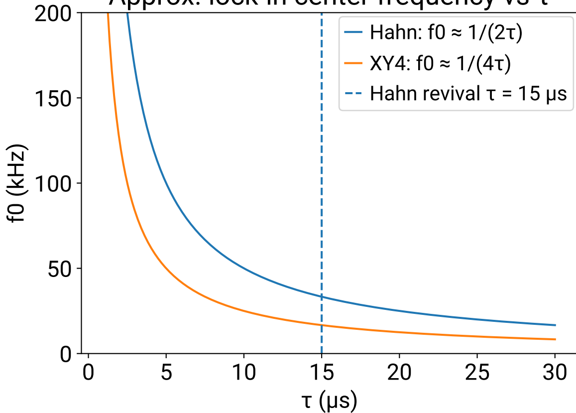
Approx. lock-in center frequency vs \tau
