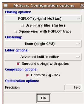
Figure 3.3.: The “configuration options” dialog in mcgui .
