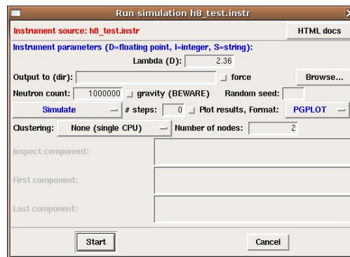
Figure 3.4.: The run dialog in mcgui .
