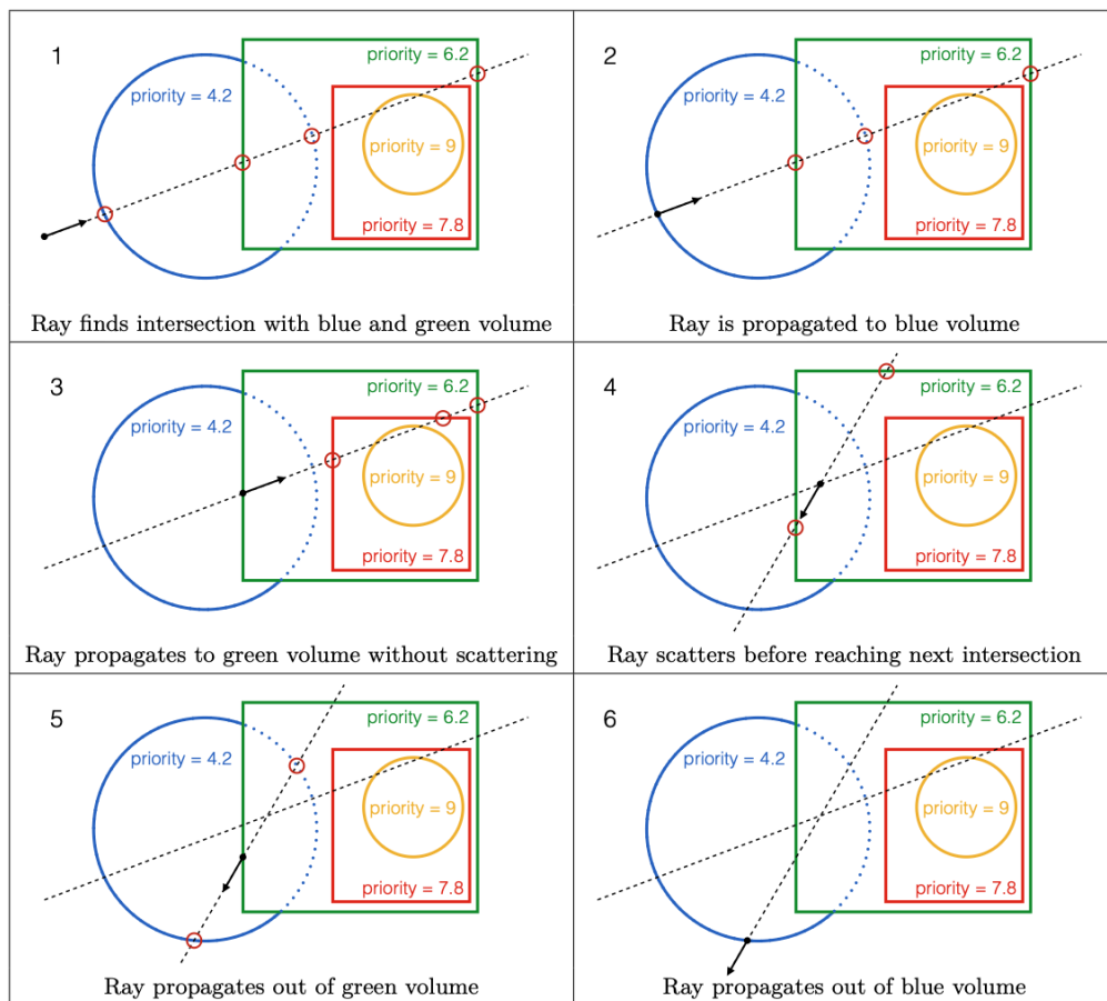
Figure 7.2.: Illustration of the Union propagation algorithm for a single scattering event between two overlapping volumes. Only intersections actually relevant given the ray's current volume are calculated at each step (the orange volume, never reachable from the ray's actual path here, is never tested).
